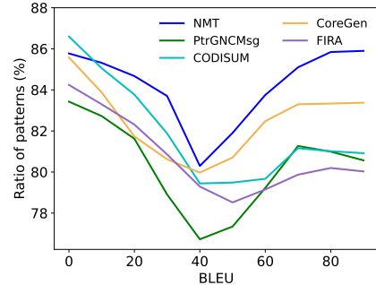
Fig. 4: The change of pattern ratio with the increase of BLEU threshold.
