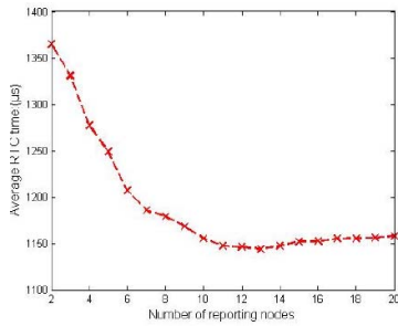
(b) The unsaturated regime
