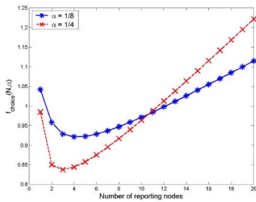
Fig. 9. Tradeoff between energy conservation and latency minimization.
