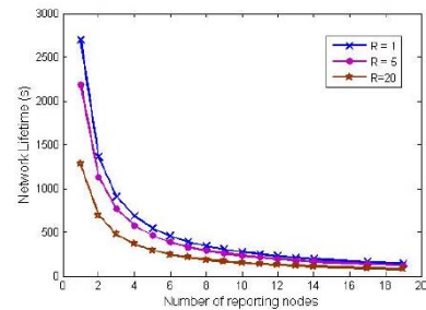
(a) The saturated regime
