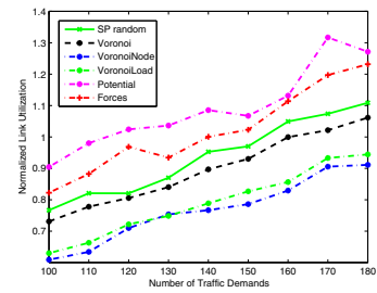
Fig. 6. Gateway placement based on iterative greedy dominating set: max link utilization
