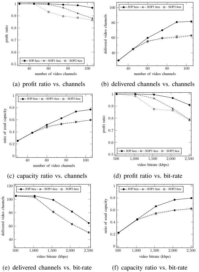
Fig. 2. Simulation Results in the French Telco-CDN (Fig. 1)
