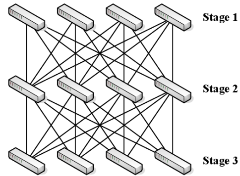
Fig. 2. Clos topology
