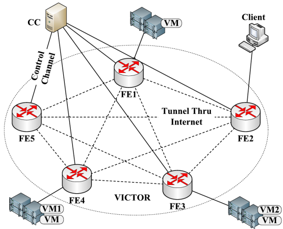
Fig. 6. VICTOR architecture.
