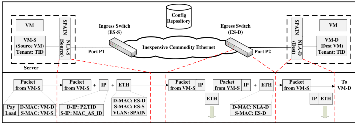
Fig. 5. NetLord architecture
