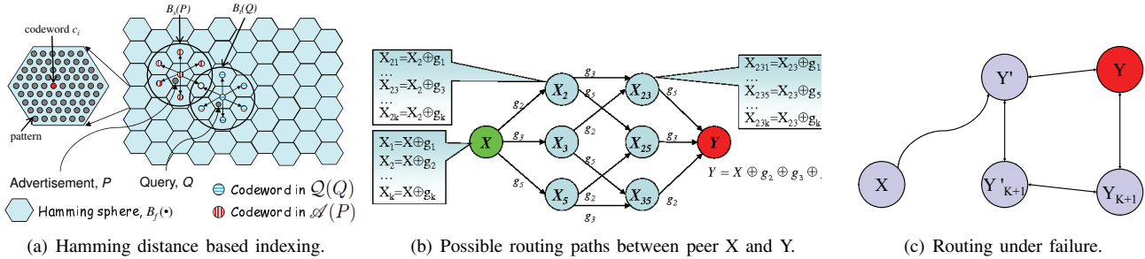
Fig. 1. Core concepts in Plexus.
