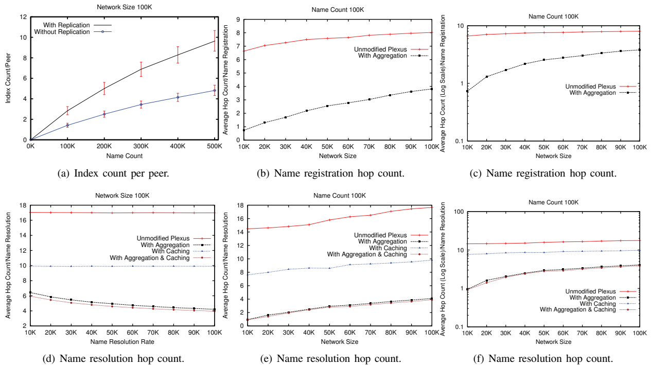
Fig. 6. Index load and hop count for name registration and resolution.
