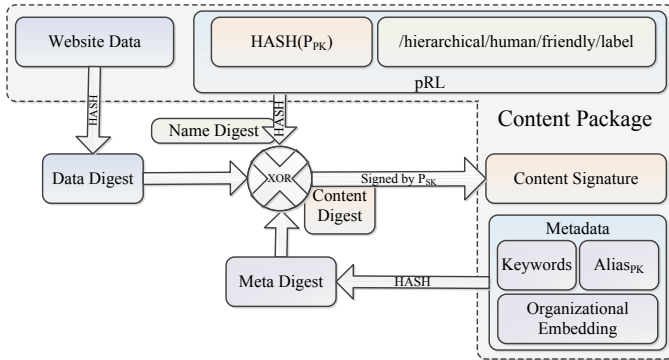
Fig. 3. Structure of a content package.
