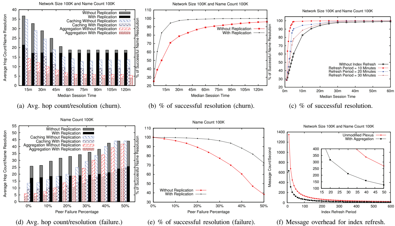
Fig. 7. Name resolution under peer churn and failure.
