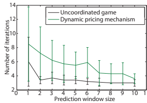
Fig. 16. Prediction horizon length vs. convergence rate.
