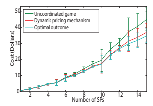
Fig. 13. Comparing the cost of NEs versus the number of players.
