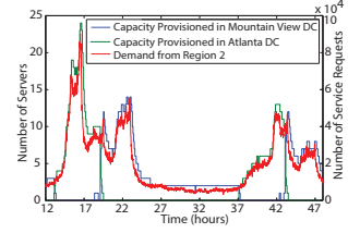
Fig. 11. Output of the greedy algorithm.
