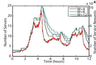
Fig. 7. Effect of prediction window size on the number of servers.
