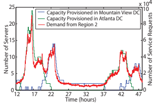
Fig. 10. Impact of price on solution quality.
