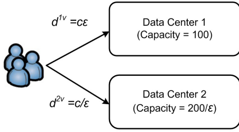
Fig. 19. Example illustrating the PoA of the game.
