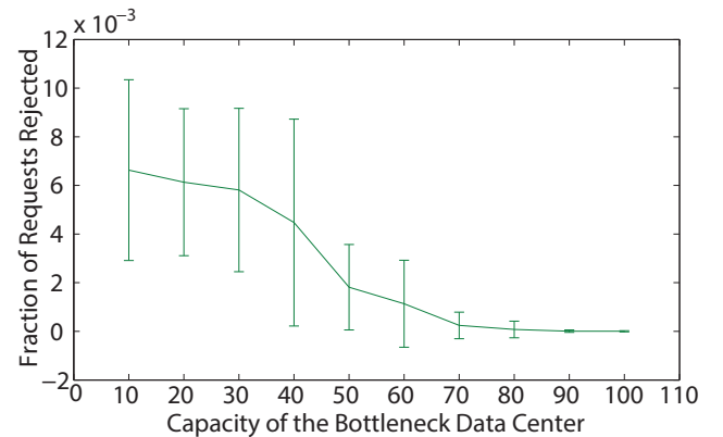
Fig. 18. Req. rejection rate vs. the capacity of the bottleneck DC.
