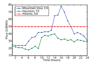
Fig. 9. Prices of electricity used in experiments.
