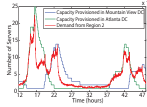
Fig. 12. Output with no reconfiguration cost and long window size.
