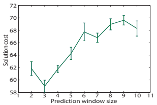
Fig. 17. Impact of prediction horizon length on the cost.
