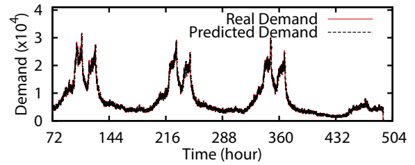
Fig. 5. Actual demand vs. Predicted demand for region 2.
