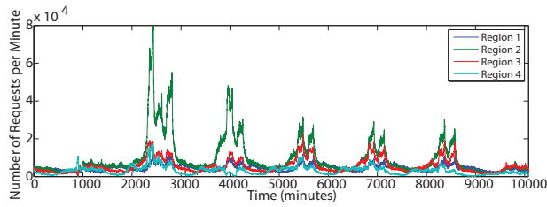
Fig. 3. HTTP requests in the Worldcup 98 dataset.
