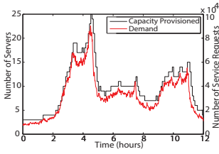
Fig. 6. Response to demand fluctuation.
