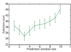
Fig. 8. Effect of prediction horizon on the solution cost.
