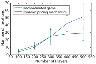
Fig. 14. Number of players vs. convergence rate.
