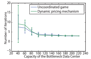
Fig. 15. Capacity of the Bottleneck DC vs. convergence rate.
