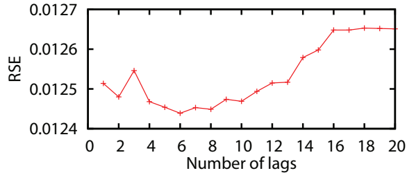
Fig. 4. Prediction accuracy vs. number of lags used.
