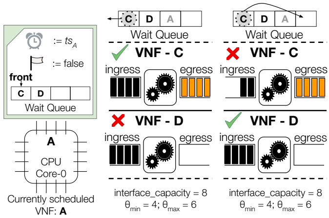
(a) State of data structures initialization (b) VNF at the queue after front satisfies the selection criteria (c) VNF at the queue front does not satisfy the selection criteria
