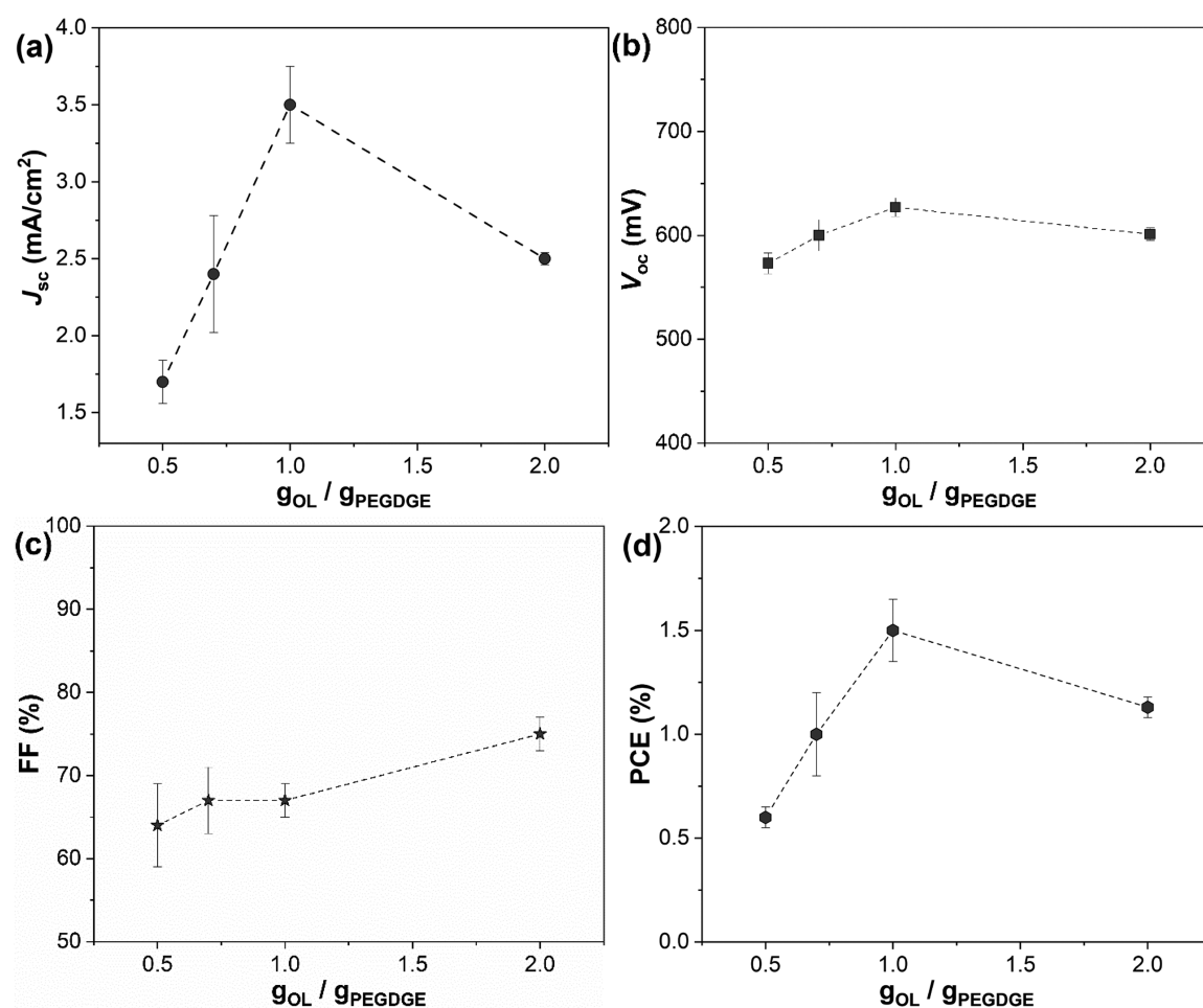
Figure 6. PV parameters for aqueous DSSCs assembled with lignin-based QS electrolytes at varying OL/PEGDGE weight ratio: (a) J_{sc} ; (b) V_{oc} ; (c) FF; (d) PCE. Each point represents the average of 5 devices, measured under 1 sun AM 1.5G irradiation (error bars represent the standard deviation).
