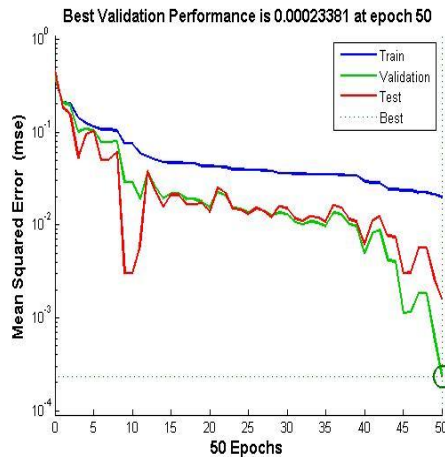
Figure 6. Performance plot for the mean square error versus the number of epochs
