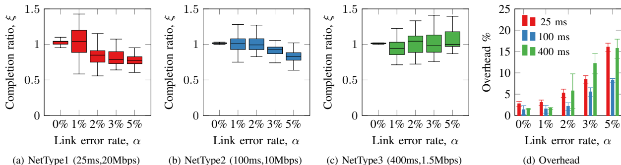
Fig. 6. Completion time ratio for the 3 scenarios under different amount of random losses for the HTTP/2 transfer (flickr.com).
