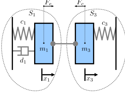
Figure 6: A multi-body system coupled by a mass-less link.
