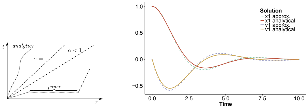
(a) Classification of time constraints in simulation. Based on [191][260].
