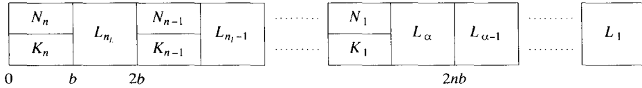
Fig. 7. A schedule for P2|fix_j|\sum w_j C_j with \sum w_j C_j \leq y .
