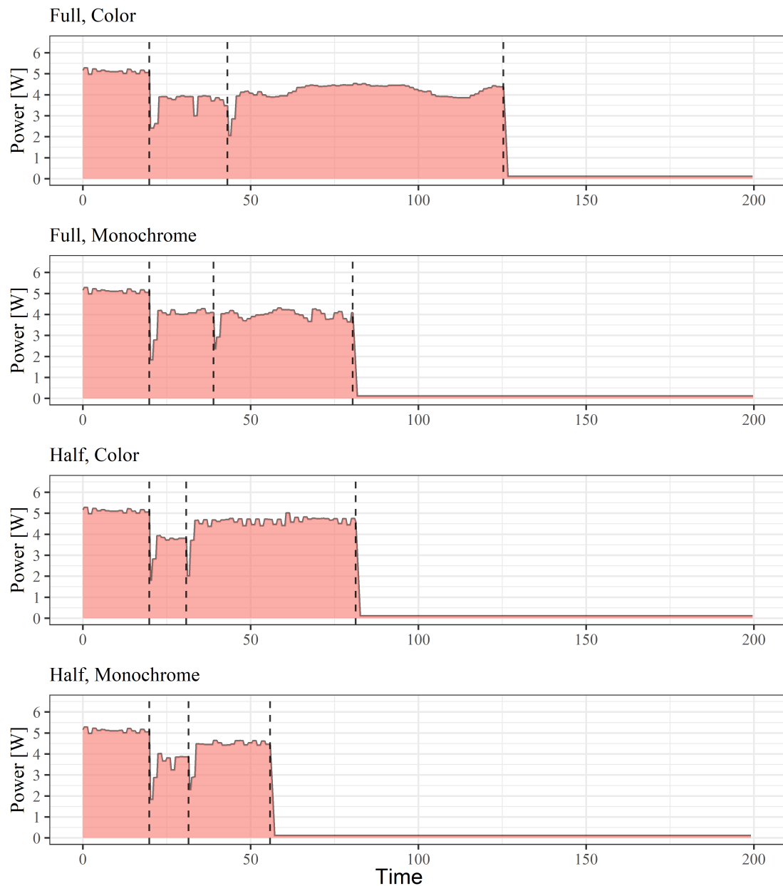
Figure 11. Power consumption for the first 200 s of a 15-min measurement cycle with a Raspberry Pi 4 at Full and Half resolution with color and monochrome images. The area under each curve represents the energy consumed during each measurement cycle.
