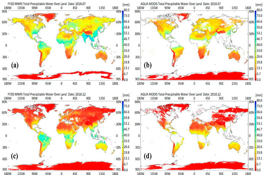
Figure 11. Comparison of monthly average TPW between FY3D MWRI and Aqua Modis in spatial scale. The monthly average TPW from FY-3D MWRI are shown for July 2018 (a) and December 2018 (c); (b) and (d) show the monthly average TPW from Aqua MODIS for July 2018 and December 2018, respectively.
