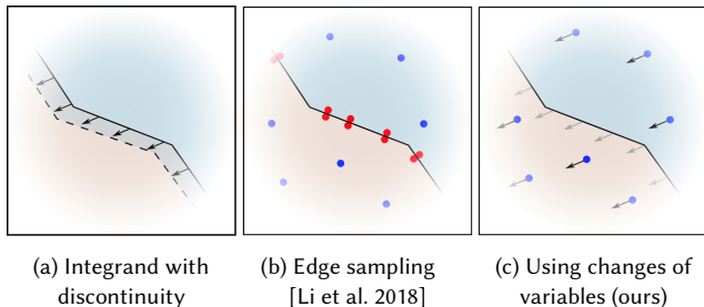
Fig. 2. (a): Integrands in physically based rendering have discontinuities whose location depends on scene parameters such as object positions. (b): In previous work [Li et al. 2018], the gradients of these integrals were estimated by sampling pairs of paths around the important silhouette edges in each integrand (red dots) in addition to standard Monte Carlo samples (blue dots). (c): We bypass the costly task of sampling visible silhouette edges by using changes of variables such that the discontinuities do not move with respect to the Monte Carlo samples for infinitesimal changes of scene parameters. This leads to Monte Carlo estimates that can be differentiated using ordinary techniques, for instance using automatic differentiation.
