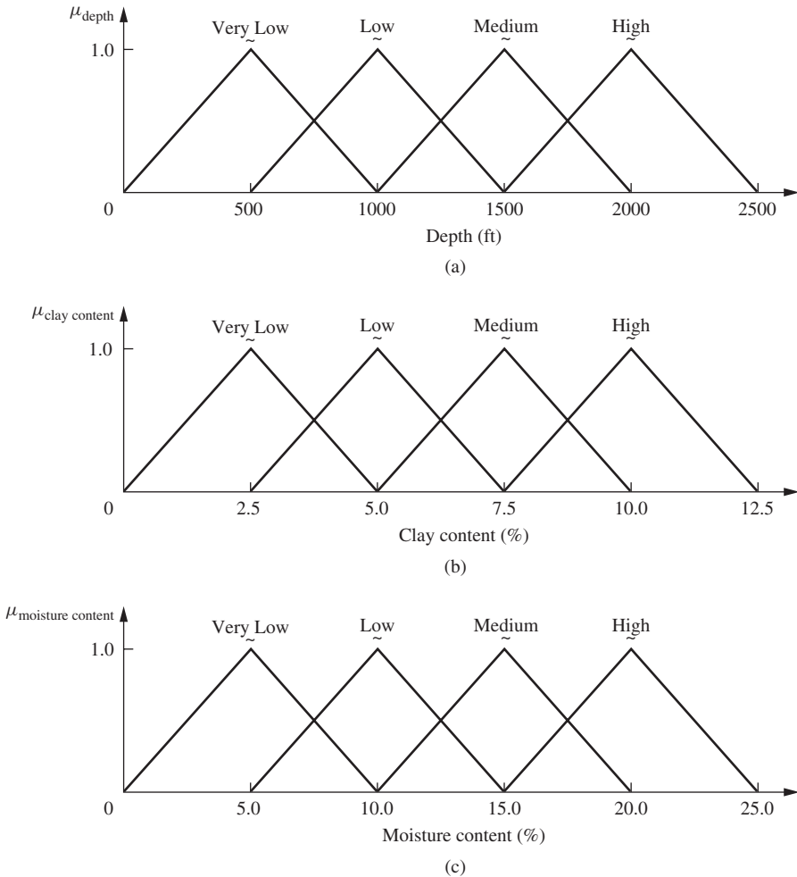
FIGURE P11.8
