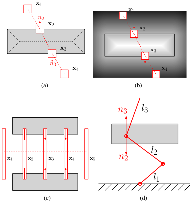
Fig. 13. Illustration of typical reasons for trajectory optimization to get stuck in local optima that are not collision-free. (a) The gradient based on penetration depth may push waypoints in inconsistent directions. (b) The gradient based on distance fields has the same problem. (c) When a robot collides simultaneously with multiple obstacles, the robot may get stuck in an infeasible local optimum as different obstacles push the robot in different directions. (d) For a robot with multiple links, the gradient may result in inconsistent directions for different links. x_i in these figures denote configurations at different time steps along the trajectory.
