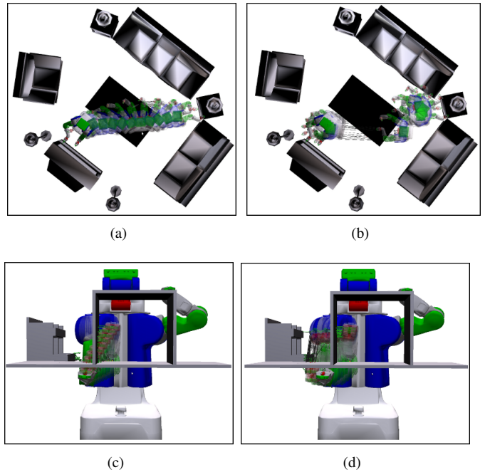
Fig. 12. Failure cases when using TrajOpt. (a) shows the initial path for full-body planning. (b) is the trajectory optimization outcome, which is stuck in an infeasible condition. (c) shows the initial path for the arm planning and the collision cannot be resolved in the final trajectory shown in (d).
