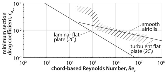
Figure 2. Minimum section drag coefficient versus Reynolds number. 7
