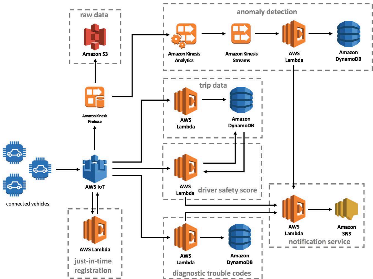
Figure 1: The connected vehicle solution architecture
