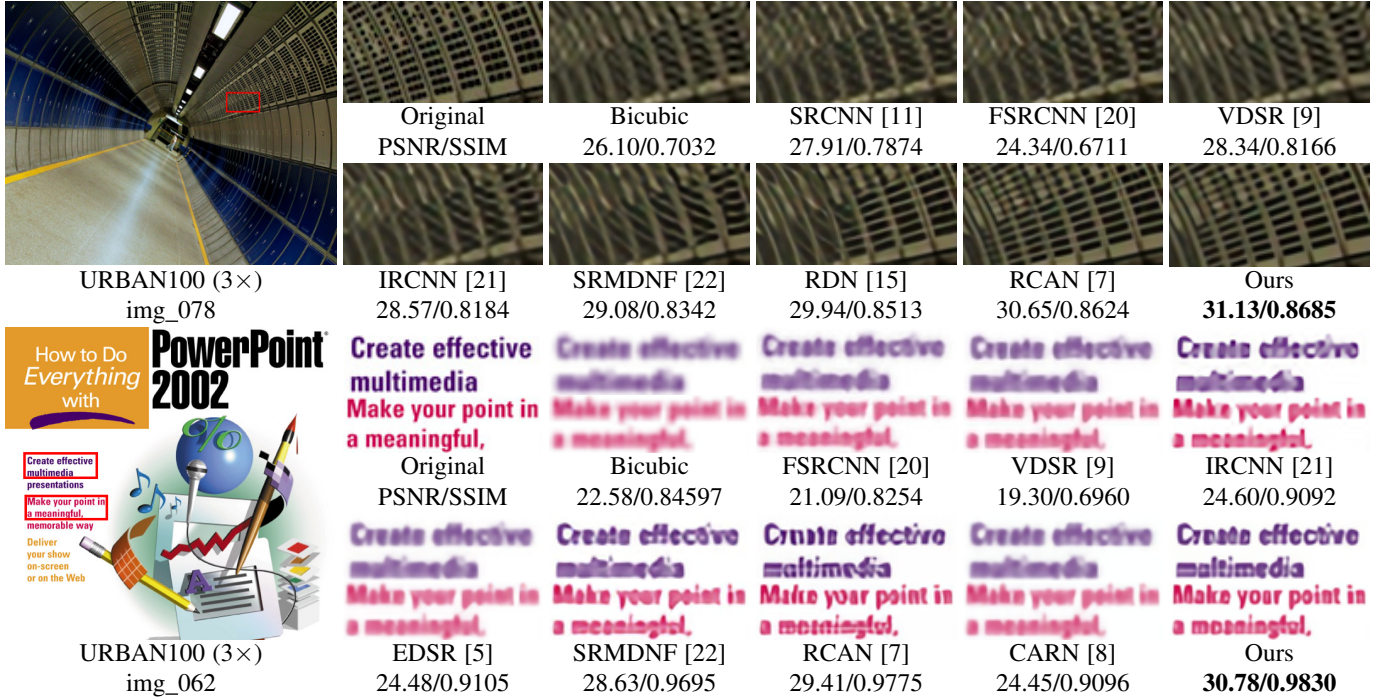
Fig. 8. Blur-Downscale (BD) degradation. Comparison on sample images with sharp edges and texture, taken from URBAN100 and SET14 datasets for the scale of 3×. The sharpness of the edges on the objects and textures restored by our method is the best.
