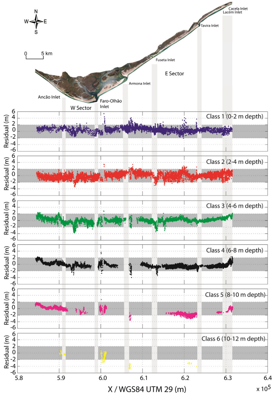
Fig. 3. Spatial distribution of the residual between Z_{LSatS} and Z_{LiDAR} along X coordinate WGS84 UTM29 for different depth classes. Vertical grey bands represent the inlet areas. Horizontal dark-grey bands represent residuals less than 2 m. The smaller amount of data at greater depths results from LiDAR data limitations (see main text Section 3.2).
