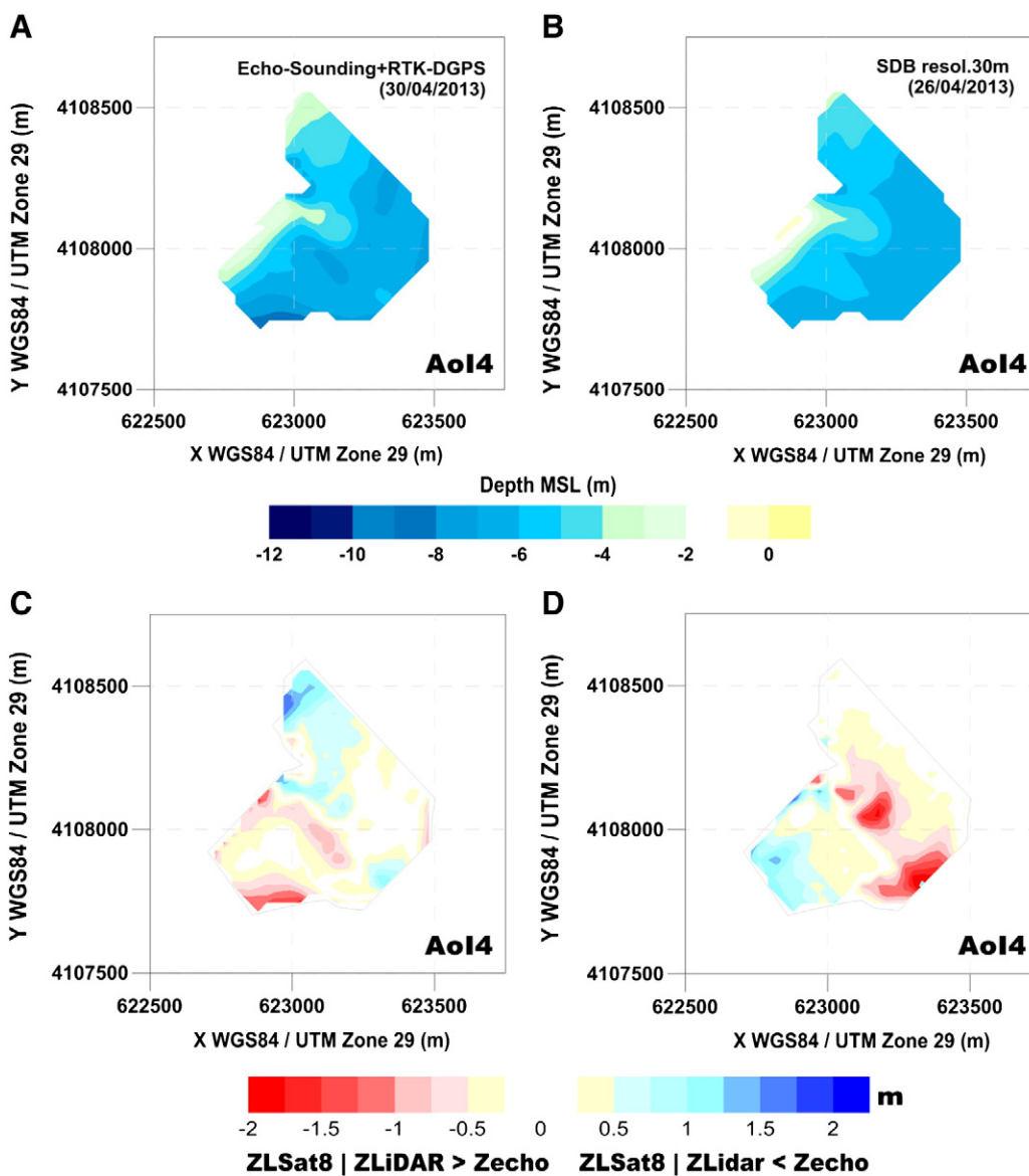
Fig. 12. (A) Aol4 bathymetry contour map acquired using an echo-sounder synchronised with a RTK-DGPS in and around Tavira Inlet on 30 April 2013. (B) Satellite-derived bathymetry (SDB) contour map (Bm3) with a 30-m resolution. (C) Difference map between A and B. (D) Difference map between LiDAR 05/2011 and SDB data derived from the Landsat 8 image of 26 April 2013; the red/blue values signify that accretion/erosion has occurred, respectively.
