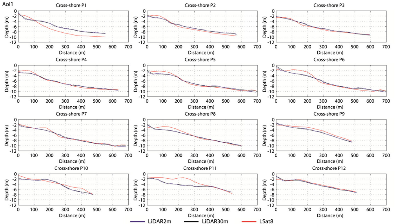
Fig. 6. AoI1 nearshore cross-profiles spaced by 1000 m and extracted from bathymetric contour maps Bm1, Bm2, and Bm3.
