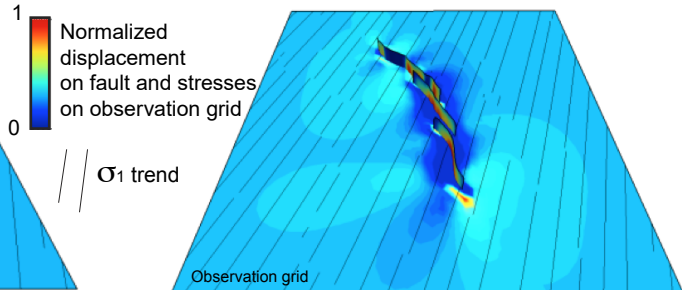
(b) Maximum Coulomb's shear stress
