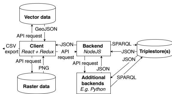
Figure 2. General architecture of SAMPO-UI.
