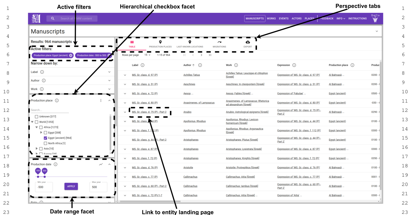
Figure 6. A selection of SAMPO-UI components for building a faceted search perspective of a semantic portal.
