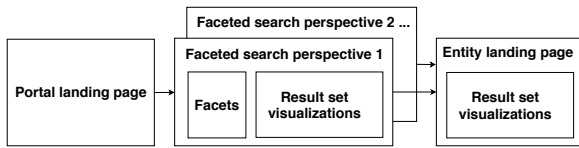
Figure 5. Main views of a semantic portal, using the default structure provided by the Sampo-UI framework. The arrows depict navigation links between the views.
