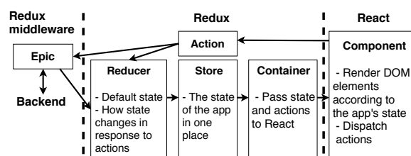
Figure 3. SAMPO-UI client architecture based on the strict unidirectional data flow of Redux integrated with React components.
