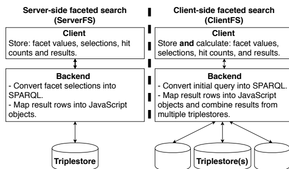
Figure 4. Faceted search architecture options of SAMPO-UI.
