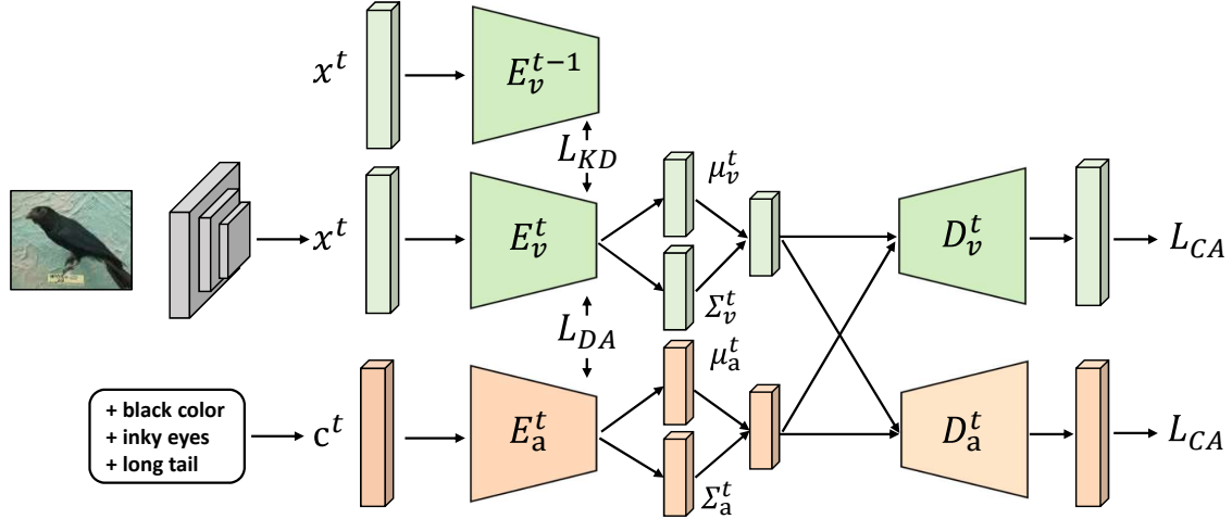
Figure 2: The framework of our proposed method in the t^{th} training stage, which consists of two VAEs and a trained encoder of visual modality in the (t - 1)^{th} training stage. Given an image, the feature extractor captures its visual feature x^t , which is mapped into the latent space as \mu_v^t and \Sigma_v^t . Meanwhile, the corresponding semantic embedding c^t is mapped into the latent space as \mu_a^t and \Sigma_a^t . Aiming to achieve latent distribution alignment, the Wasserstein distance between the latent distributions ( \mathcal{L}_{DA} ) is minimized in the training stage. Then, the cross-alignment loss ( \mathcal{L}_{CA} ) is employed to guarantee the latent distributions aligned through cross-modal reconstruction. Besides, we leverage knowledge distillation ( \mathcal{L}_{KD} ) to transfer knowledge obtained from previous tasks to current task.
