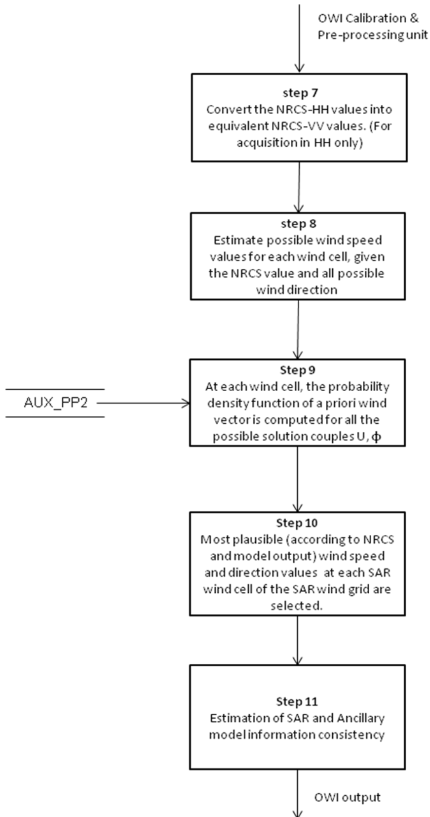
Figure 5-5 Inversion Unit Flowchart (before IPF 2.91)
