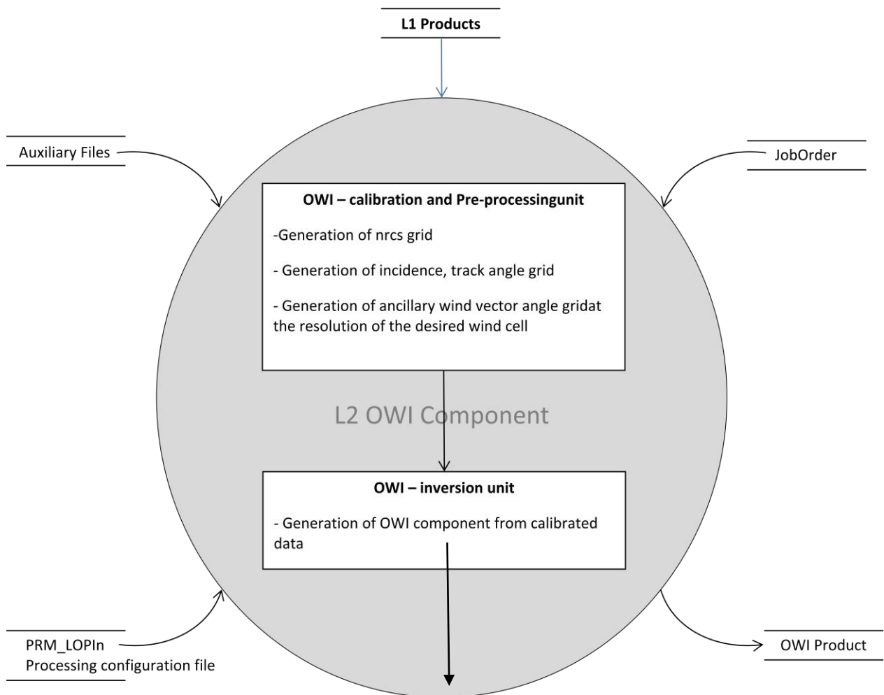
Figure 4-1 High Level OWI Processing Algorithm
