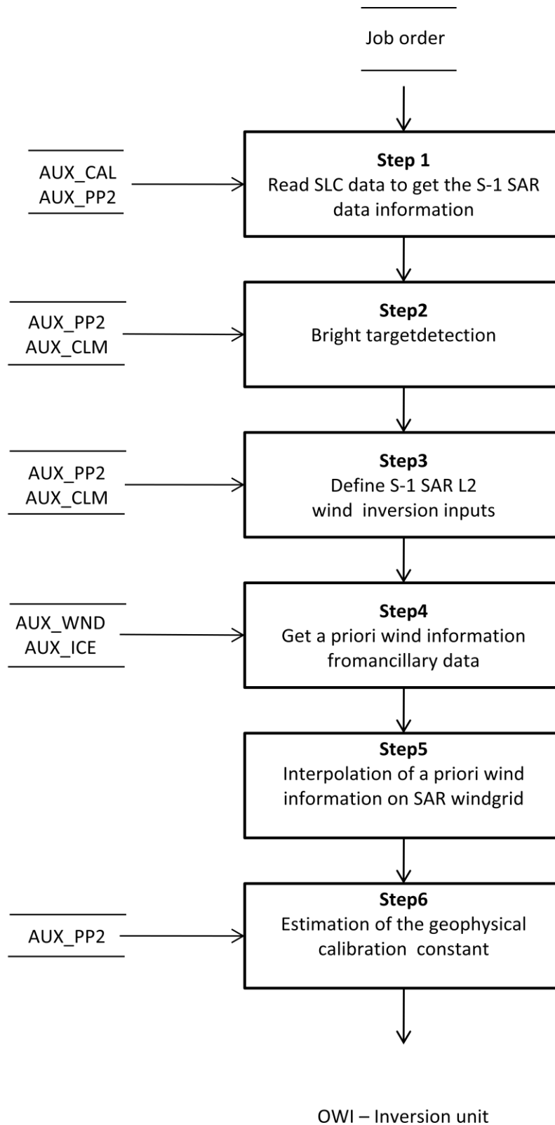
Figure 5-1 Calibration and Pre-processing Unit Flowchart
