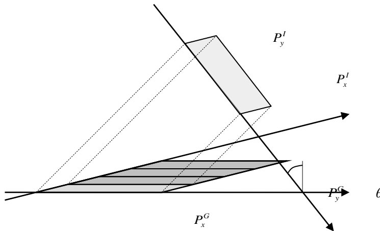
Figure 5-2 Data Products Not Converted from Slant Range to Ground Range
