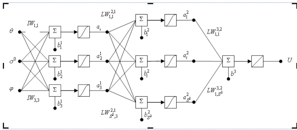
Figure 9-2 Neural Network Architecture for the Implementation of the Inverse CMOD Scattering Models
