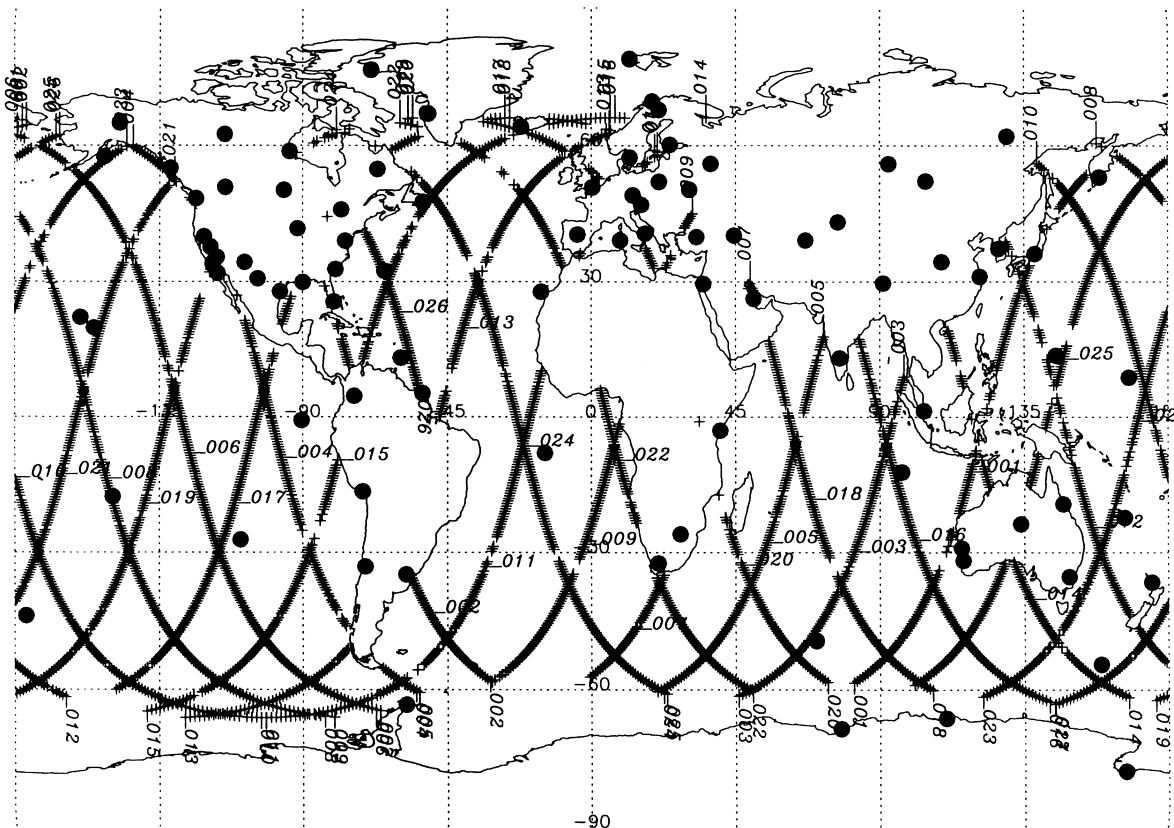
Fig. 5. Locations of global network receivers (●) and TOPEX ground tracks for 20 July 1998. TOPEX pass numbers are shown.
