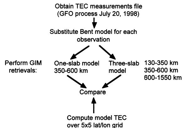
Fig. 2. Method for assessing three-dimensional retrievals against a two-dimensional model run. The obliquity factor for the single slab model is for a constant density slab extending from 350 to 600 km.
