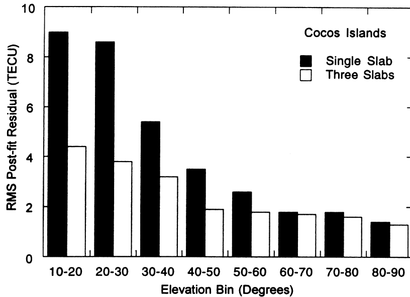
Fig. 8. Postfit residuals for the Cocos Islands site binned by elevation angle.
