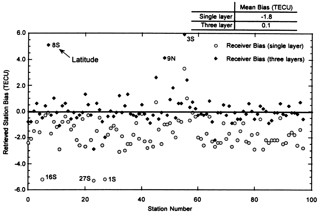
Fig. 3. Comparison of retrieved receiver biases for the single and multilayer approaches using simulated data. Ground truth values are all zero. Sites with the largest error values are labeled by latitude.
