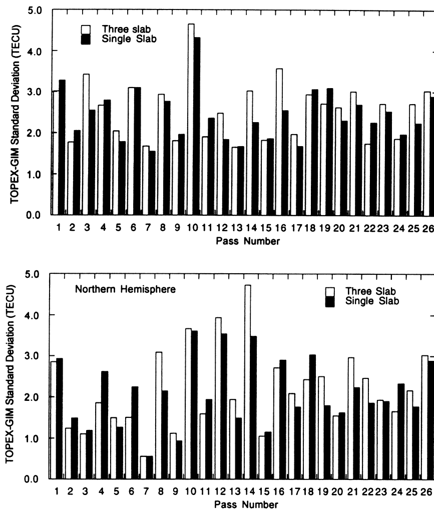
Fig. 6. Standard deviations of the differences between TOPEX and GIM plotted by TOPEX pass number for both retrieval methods. Comparisons are plotted separately for Northern (latitude > 0) and Southern (latitude < 0) regions.
