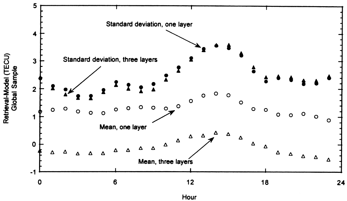
Fig. 4. Statistics on the differences between retrieved TEC and ground truth over a 5^\circ \times 5^\circ latitude/longitude global grid. Maps were updated once per hour.
