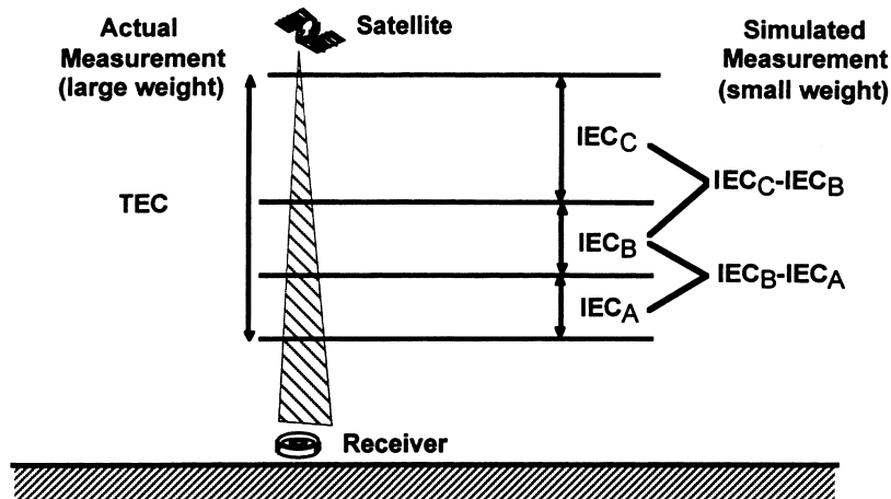
Fig. 1. Representation of what is observed using live data (TEC) versus what is generated using an electron density model: measurements of the differential integrated electron content between adjacent layers.
