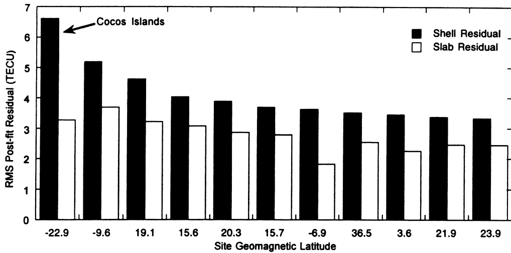
Fig. 7. Postfit residuals of slant data by site for single and multilayer methods. Only the sites with the 11 largest residuals are shown.
