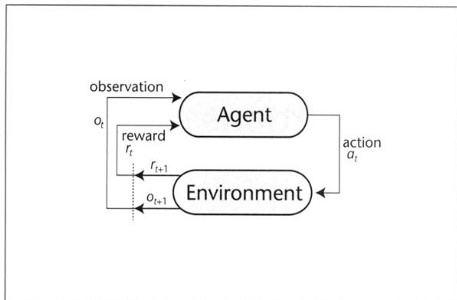
Figure 1. Interaction between an Agent and an Environment.
