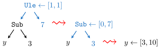
Figure 1: Processing the constraint Ule(Sub(y, 3)) in the learning stage, where constraints are processed top-down in order to derive information about the solution sets of variables ( y in this case.)
