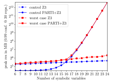
Figure 5: Peak resident memory for symbolic execution of the worst case and control programs. PARTI performs well up to a number of 16 Add expressions, when the number of individual intervals in one multi-interval surpasses 2^{16} .
