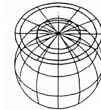
Fig. 3-16: Polar Stereographic Projection. Figure taken from [RD 3].
