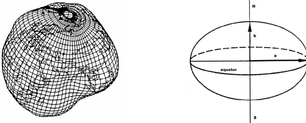
Fig. 3-13: Geoid (left), Ellipsoid (right). Figures taken from [RD 3].
