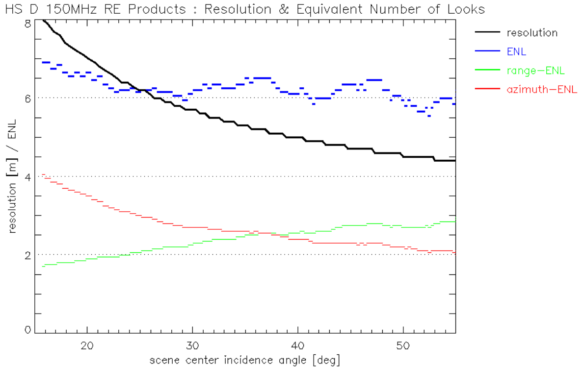
Fig. 21: High-resolution Spotlight dual polarization RE product variant for 150 MHz range bandwidth.
