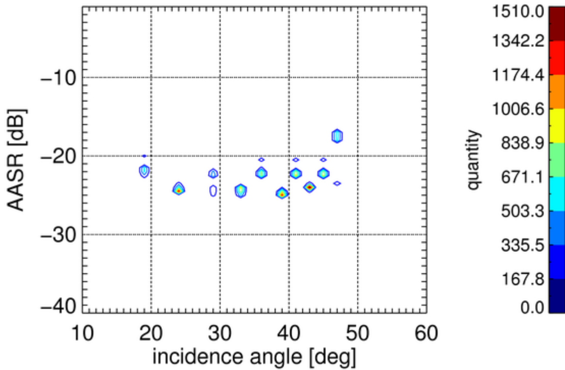
Figure 2 Simulated AASR for the statistical acquisitions. The AASR values of the worst point target within each scene are depicted as the contour lines of the two dimensional histogram over incidence angle.
