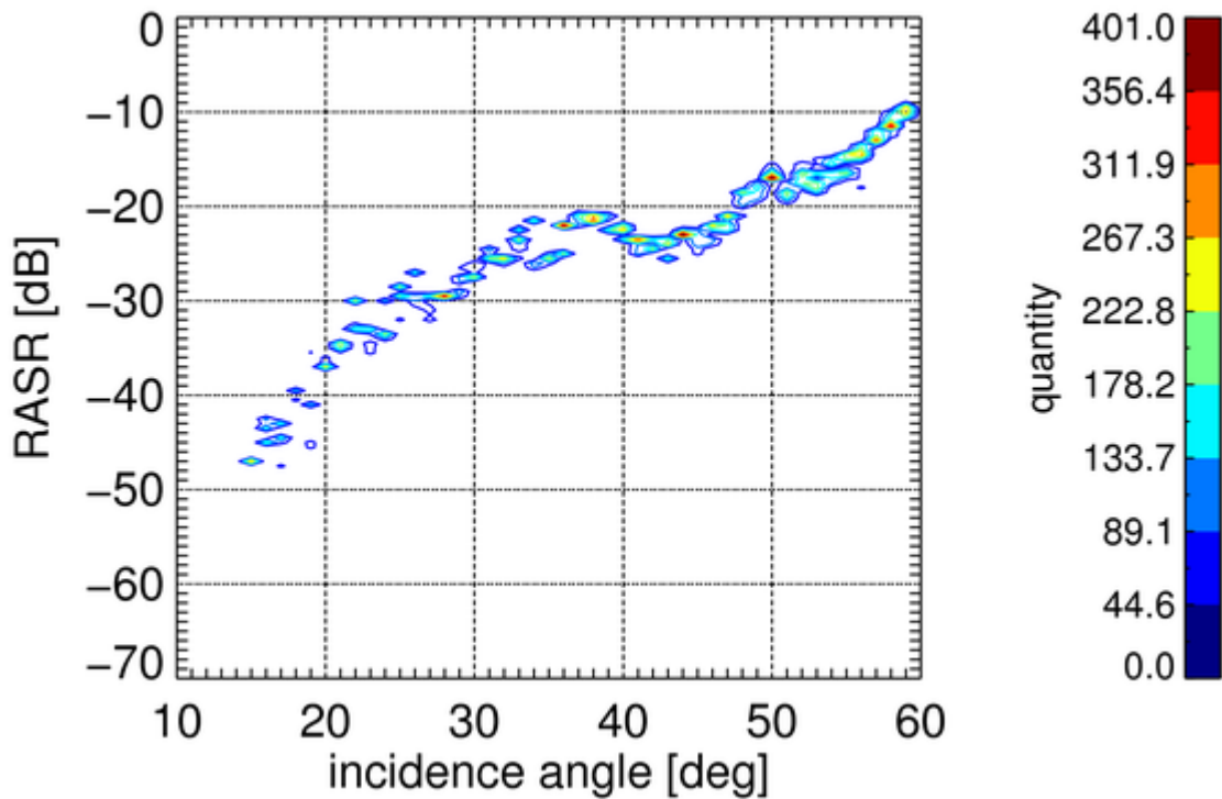
Figure 10 Simulated RASR of the worst target over range for more than 20000 statistical acquisitions. The contour lines of the two dimensional histogram are given, highlighting the dominant regions of predicted RASR.
