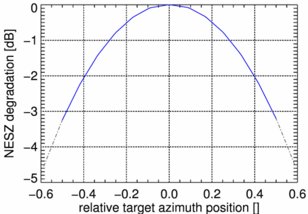
Figure 11 Degradation of the NESZ referenced to the center of the scene (blue curve). The abscissa represents the normalized position of a point target within the whole scene with scene center at zero and +/- 0.5 as the full performance azimuth extent limits. The NESZ degradation for the extended coverage areas in steep incidence angle products is indicated with the dashed-dotted line.
