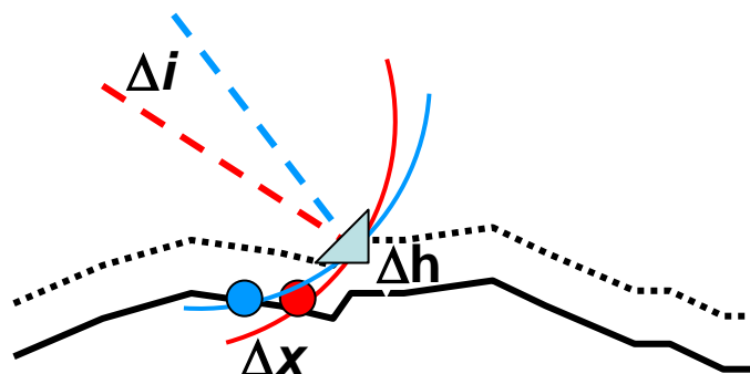
Fig. 3-8: Sketch of DEM height to location error relation for different incidence angles
