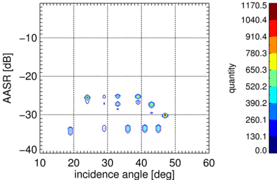
Figure 1 Simulated AASR for the statistical acquisitions. The AASR values of the best point target within each scene are depicted as the contour lines of the two dimensional histogram over incidence angle. The ten elevation beams are clearly distinguishable.
