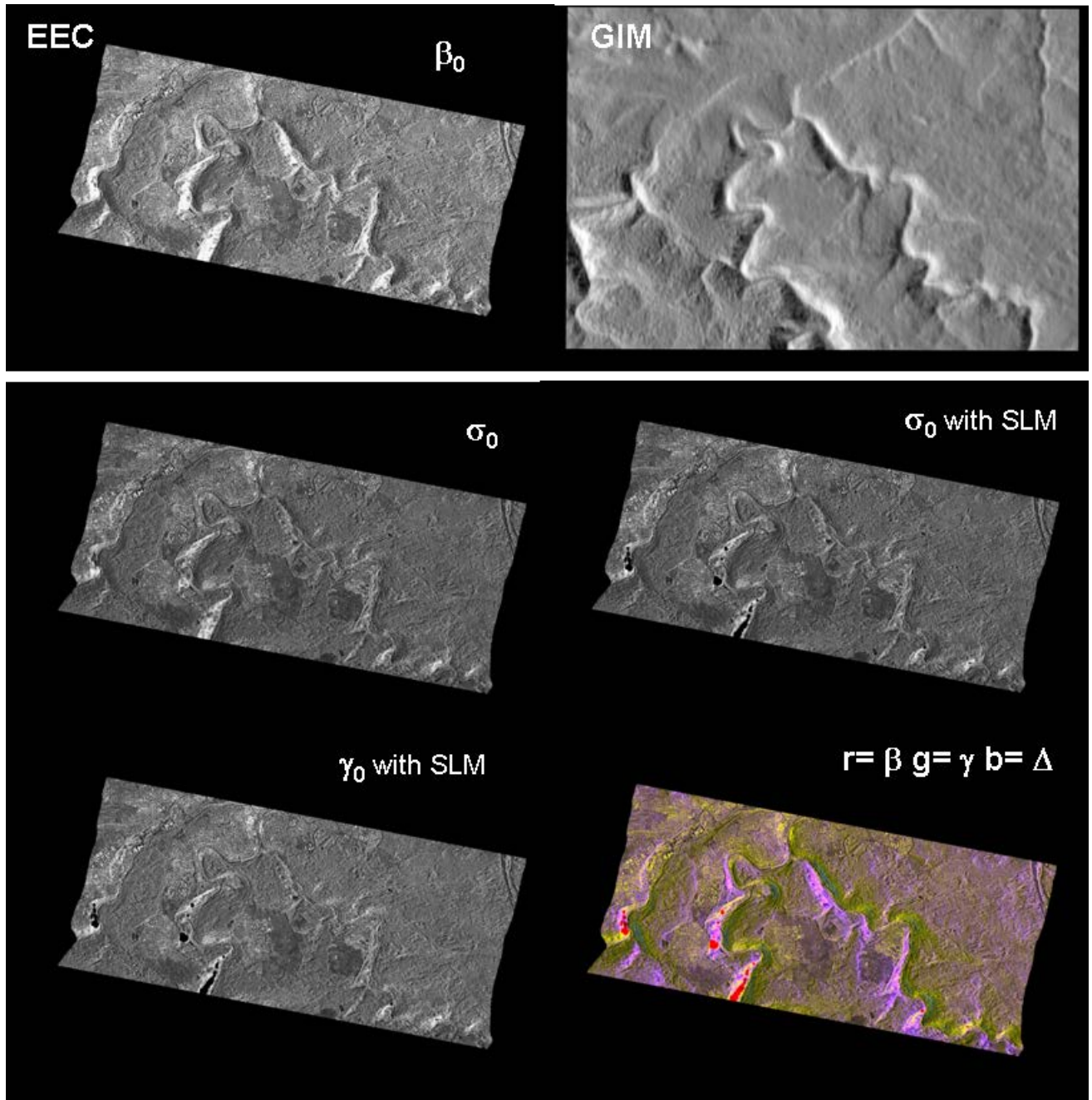
Fig. 3-12: Example for radiometric conversions using the product component GIM of a HS EEC L1b. The RGB composite indicates the differences between the beta nought and the gamma nought representation.
