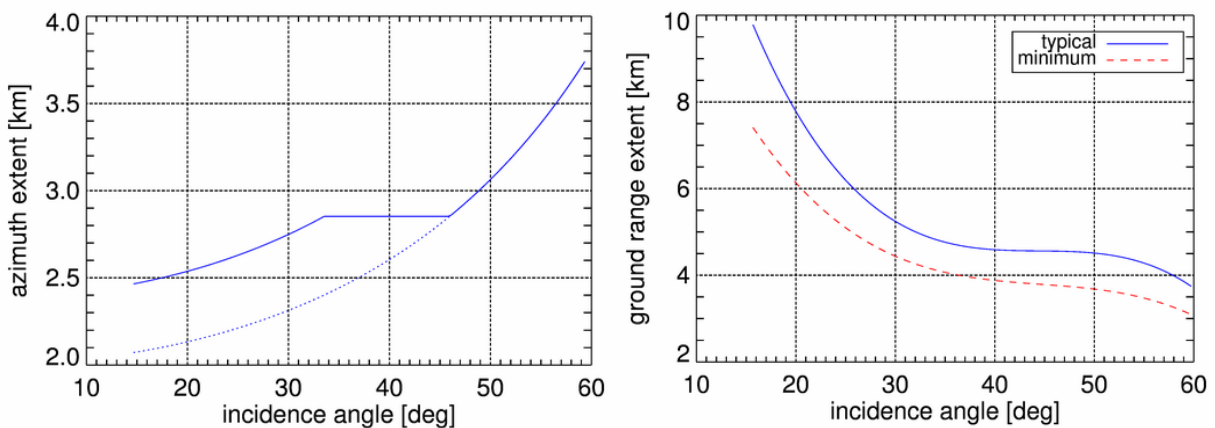
Fig. 2-7: Nominal scene extent of Staring Spotlight products in single pol 300 MHz mode for different scene center incidence angles. The lines represent typical values or lower boundaries (dashed line). The dotted line for the azimuth extent indicates the full performance extent, the solid one shows the extended coverage provided in the user products.
