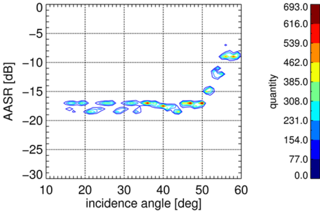
Figure 7 Simulated AASR at the azimuth scene edges of the ST products (as defined by the solid line in the azimuth extent plot) for more than 20000 statistical acquisitions. The contour lines of the two dimensional histogram are given, highlighting the dominant regions of predicted AASR.
