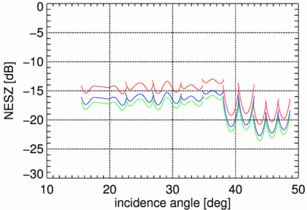
Figure 5 NESZ for the ten wide-beams. For each beam a dedicated range chirp bandwidth and duty cycle combination is used.
