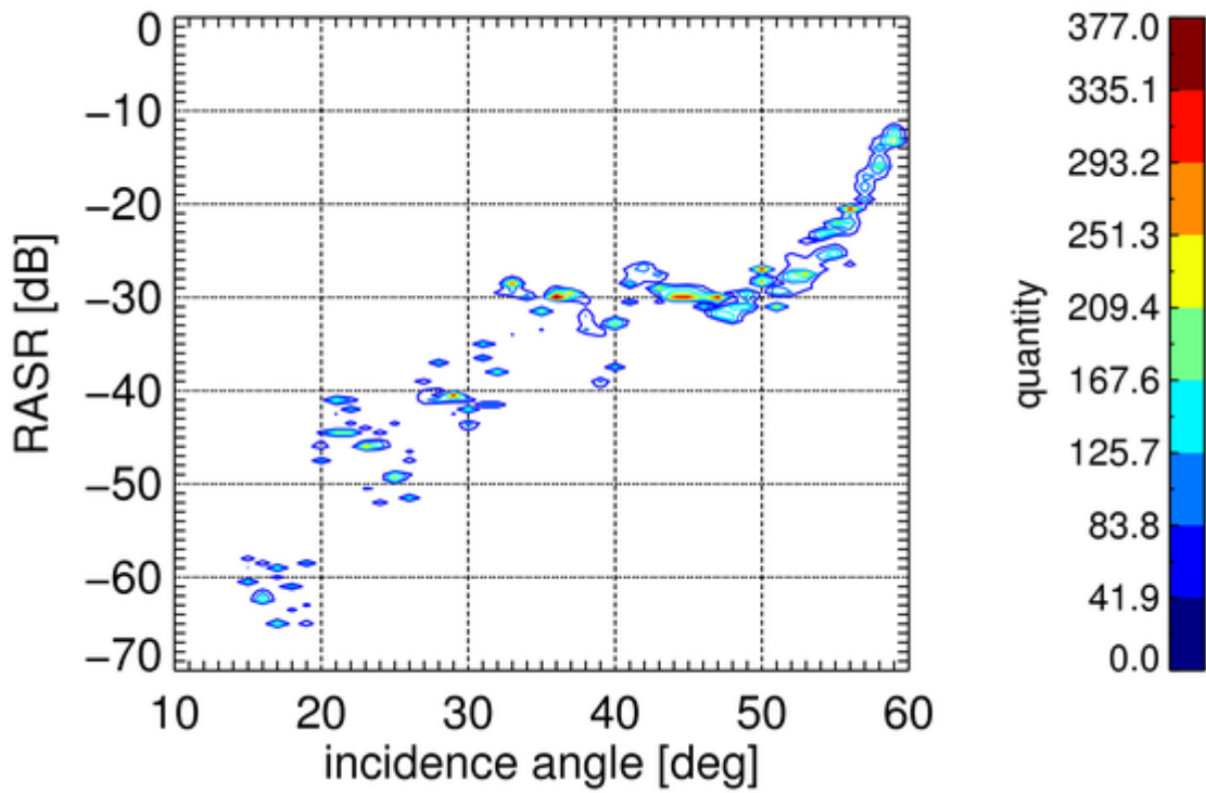
Figure 9 Simulated RASR of the best target over range for more than 20000 statistical acquisitions. The contour lines of the two dimensional histogram are given, highlighting the dominant regions of predicted RASR.
