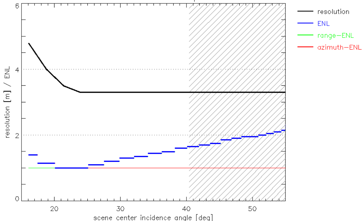
SM S 150MHz SE Products : Resolution & Equivalent Number of Looks
