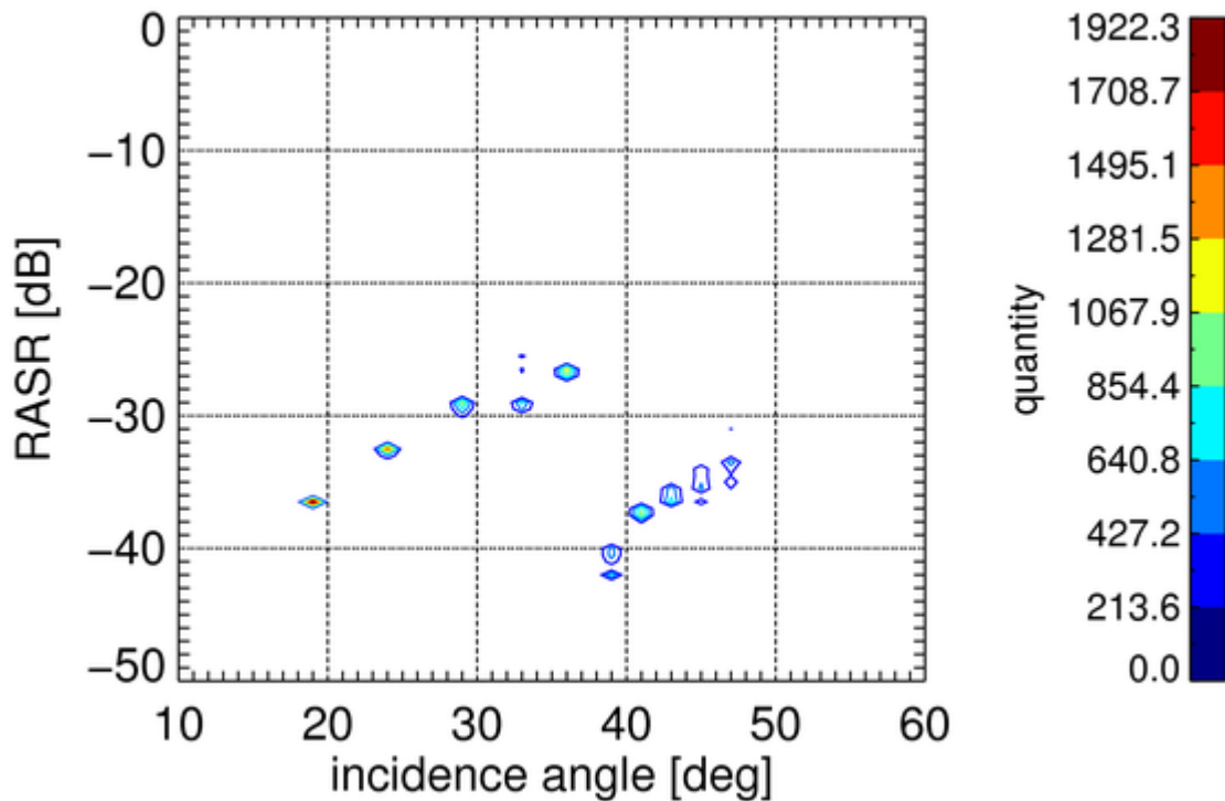
Figure 3 Simulated RASR for the statistical acquisitions. The RASR values of the best point target within each scene are depicted as the contour lines of the two dimensional histogram over incidence angle.
