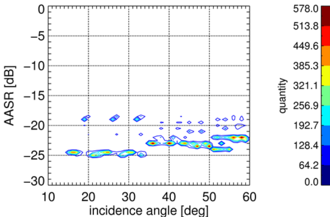
Figure 6 Simulated AASR at scene center for more than 20000 statistical acquisitions. The contour lines of the two dimensional histogram are given, highlighting the dominant regions of predicted AASR.
