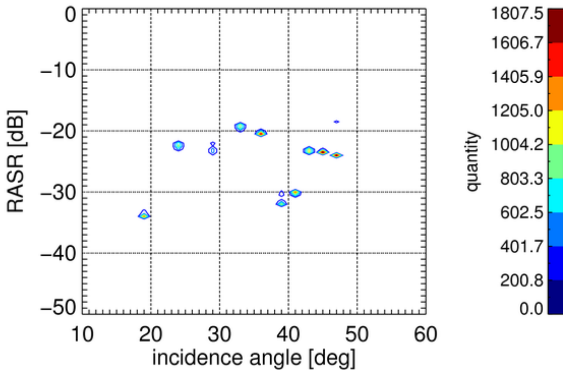
Figure 4 Simulated RASR for the statistical acquisitions. The RASR values of the worst point target within each scene are depicted as the contour lines of the two dimensional histogram over incidence angle.
