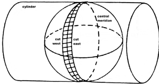
Fig. 3-15: Transverse Mercator Figure taken from [RD 3].
