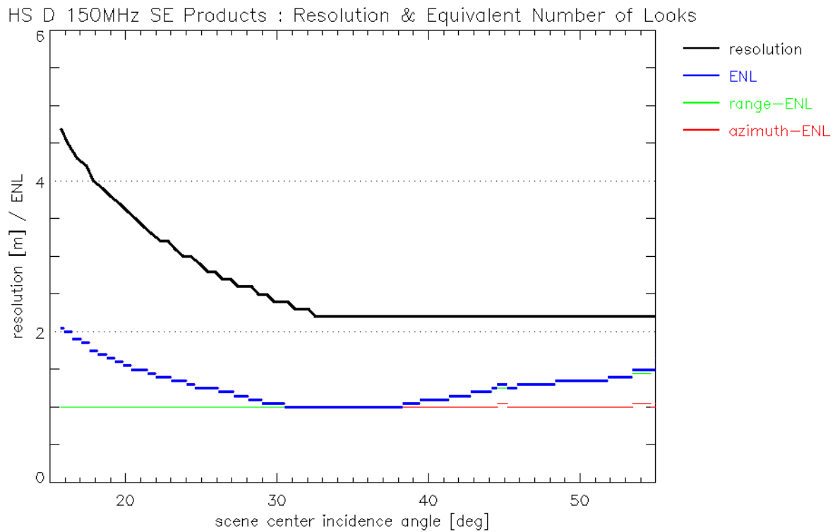
Fig. 22: High-resolution Spotlight dual polarization SE product variant for 150 MHz range bandwidth.
