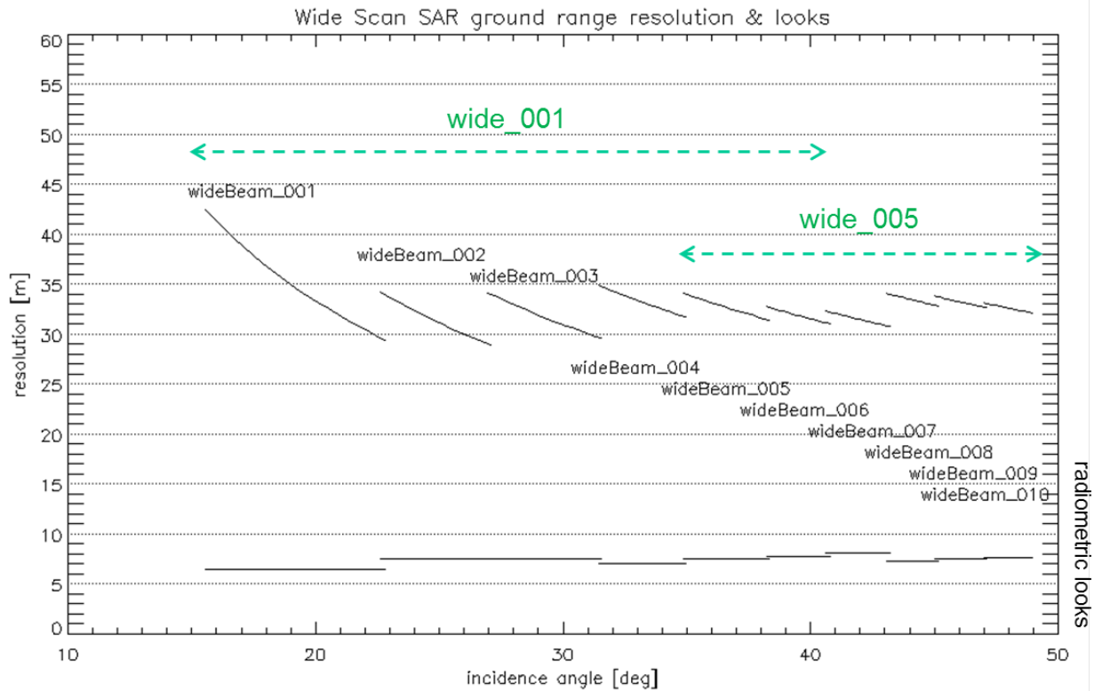
Fig. 3-6: The configured ground range resolution and radiometric looks of targets in detected six beam wide ScanSAR images (only RE variants exist for this product type). The multi-looking parameters are individually optimized for each beam of the 6-beam “wide” configurations yielding only slight variations in resolution and looks.
