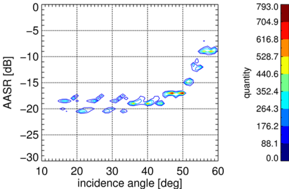
Figure 8 Simulated worst case AASR at the full performance azimuth scene limits of the ST products for more than 20000 statistical acquisitions. The contour lines of the two dimensional histogram are given, highlighting the dominant regions of predicted AASR.
