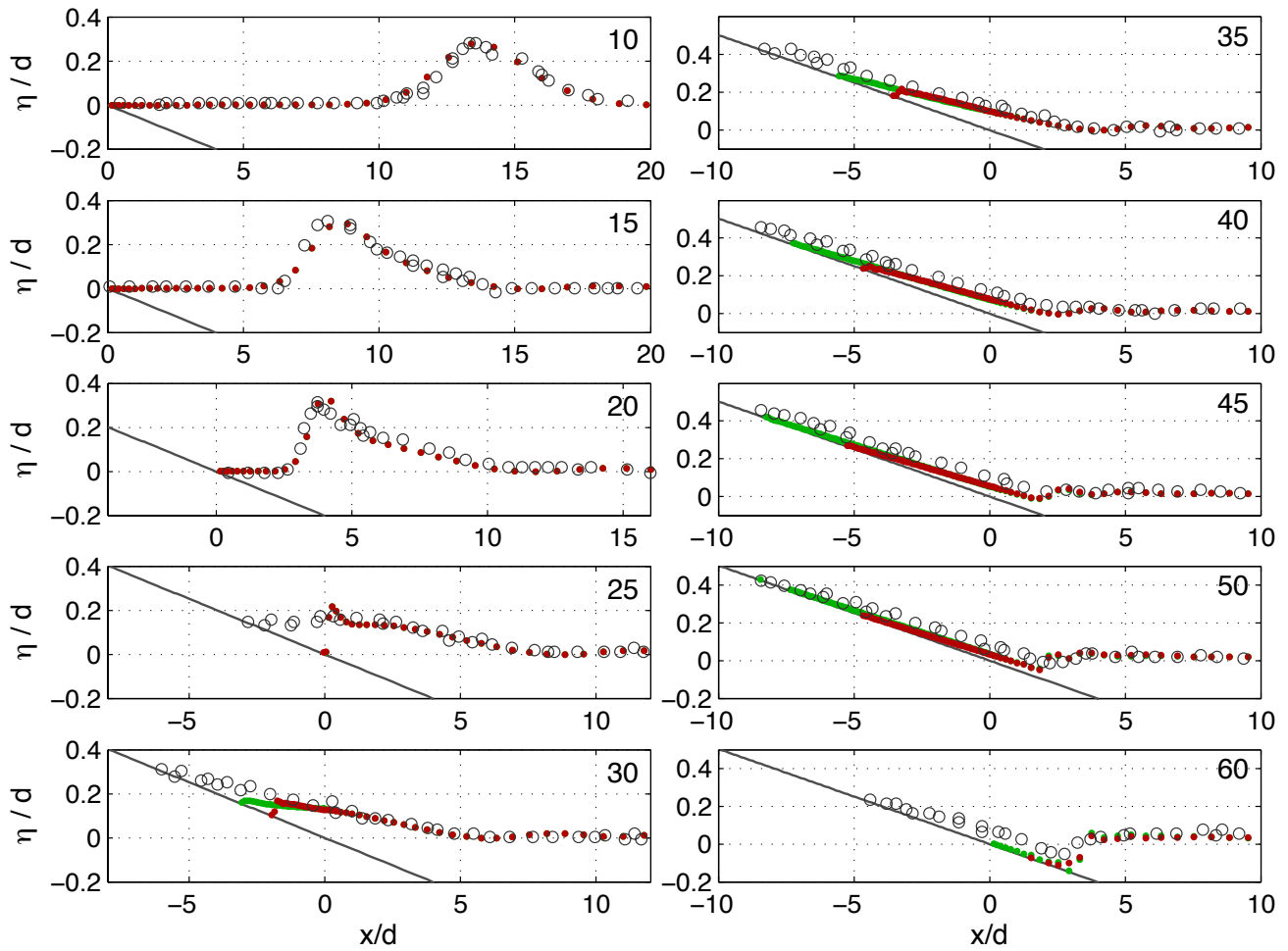
Figure 15: Water surface profiles for an initial solitary wave 0.3d high climbing up a 1:19.85 beach at different t/\tau (as written in a plot). MOST numerical solution (red) is plotted atop Cliffs solution (green), gray circles - measurements.
