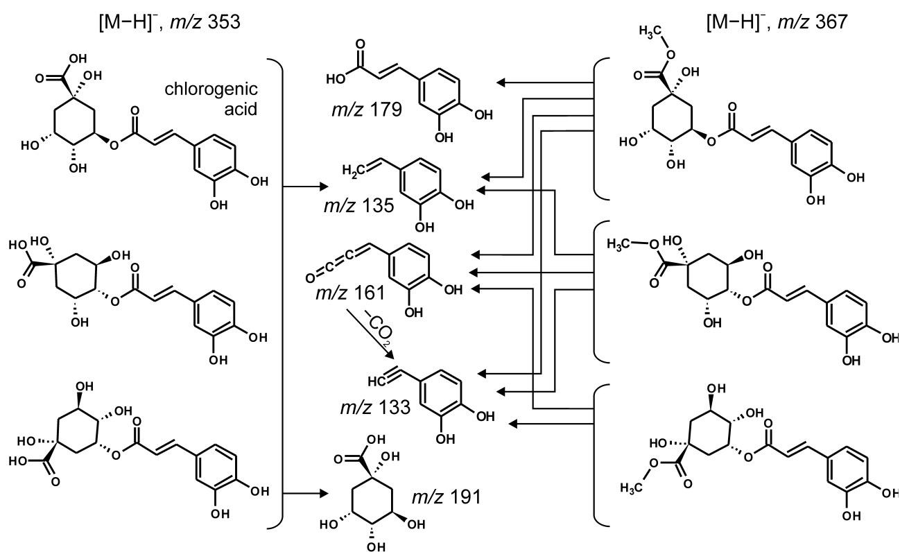
Fig. S1. Proposed structures and fragmentation pathways of chlorogenic acid isomers (left) and their methylated analogue (right)
