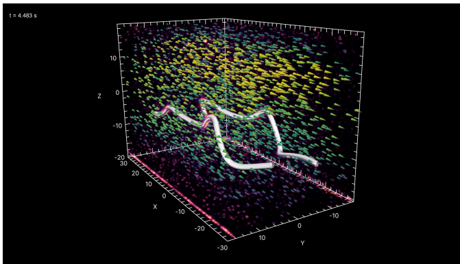
Fig. 16 Supplementary Movie S3. A movie of the vortex line tracking of the dye superimposed with PTV tracks for vortices in a pipe flow.
