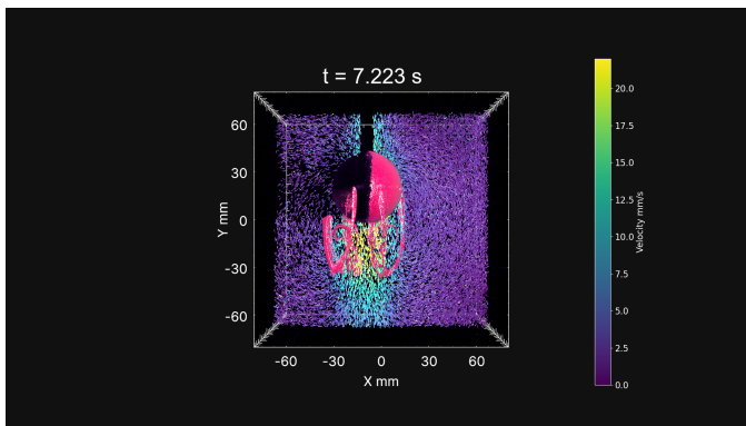
Fig. 15 Supplementary Movie S2. A movie of raw data of an isosurface of fluorescent dye overlaid with the PTV velocity field. Measurements are taken at Re = 400 .
