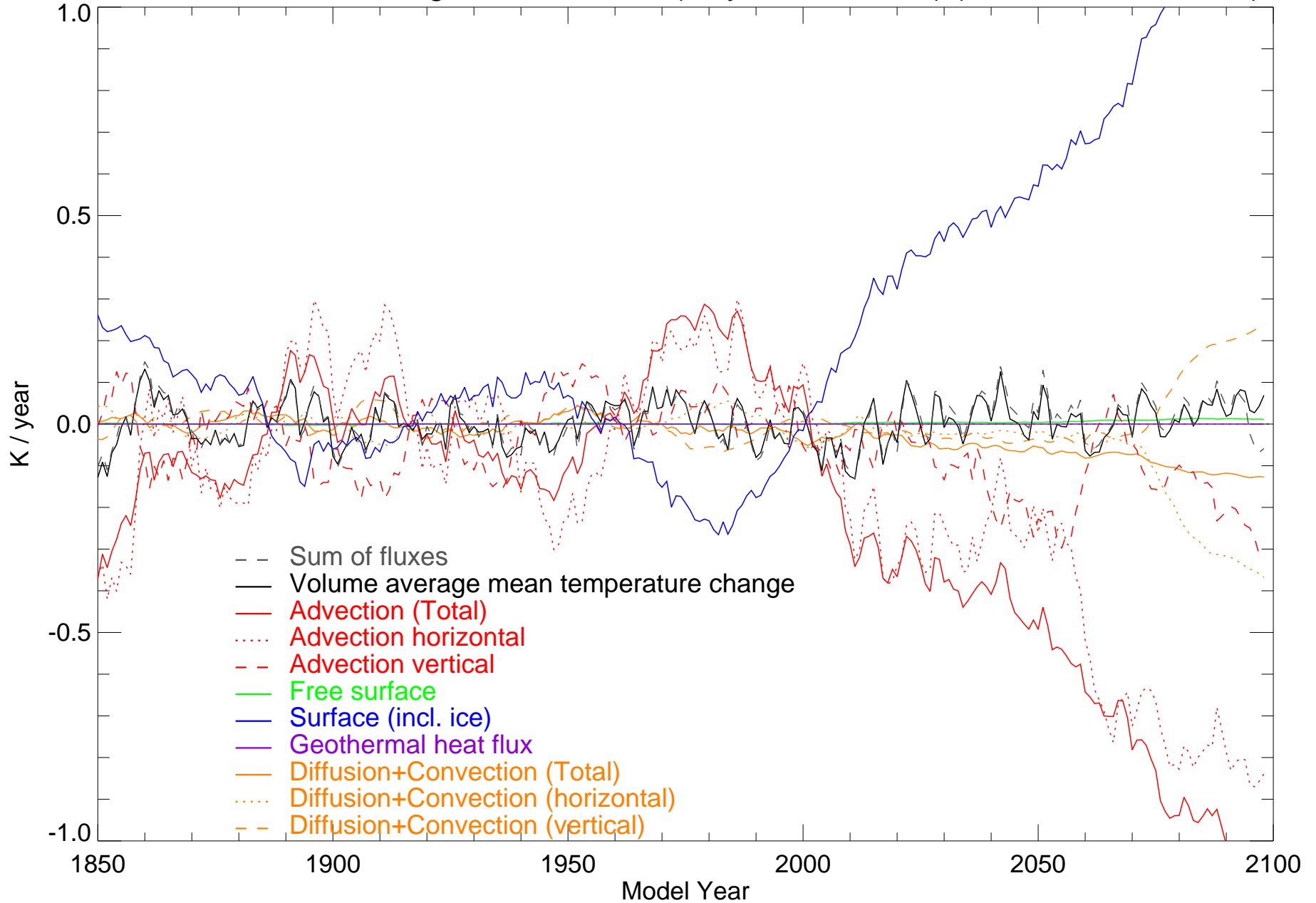
HadGEM3-GC2 WH region 0->316.77m (11 year smoothed) (anom wrt 1850-2000)
