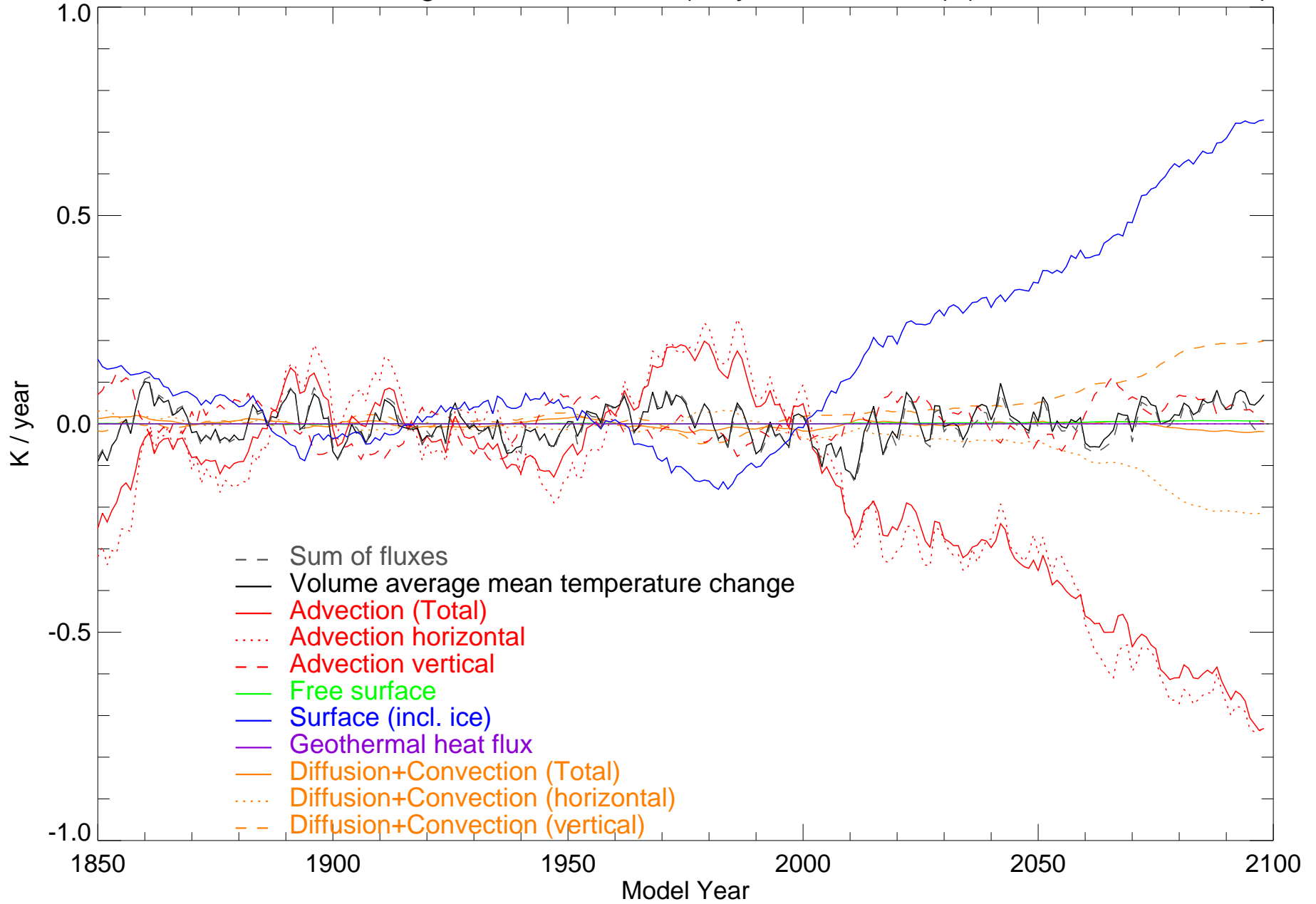
HadGEM3-GC2 WH region 0->535.991m (11 year smoothed) (anom wrt 1850-2000)
