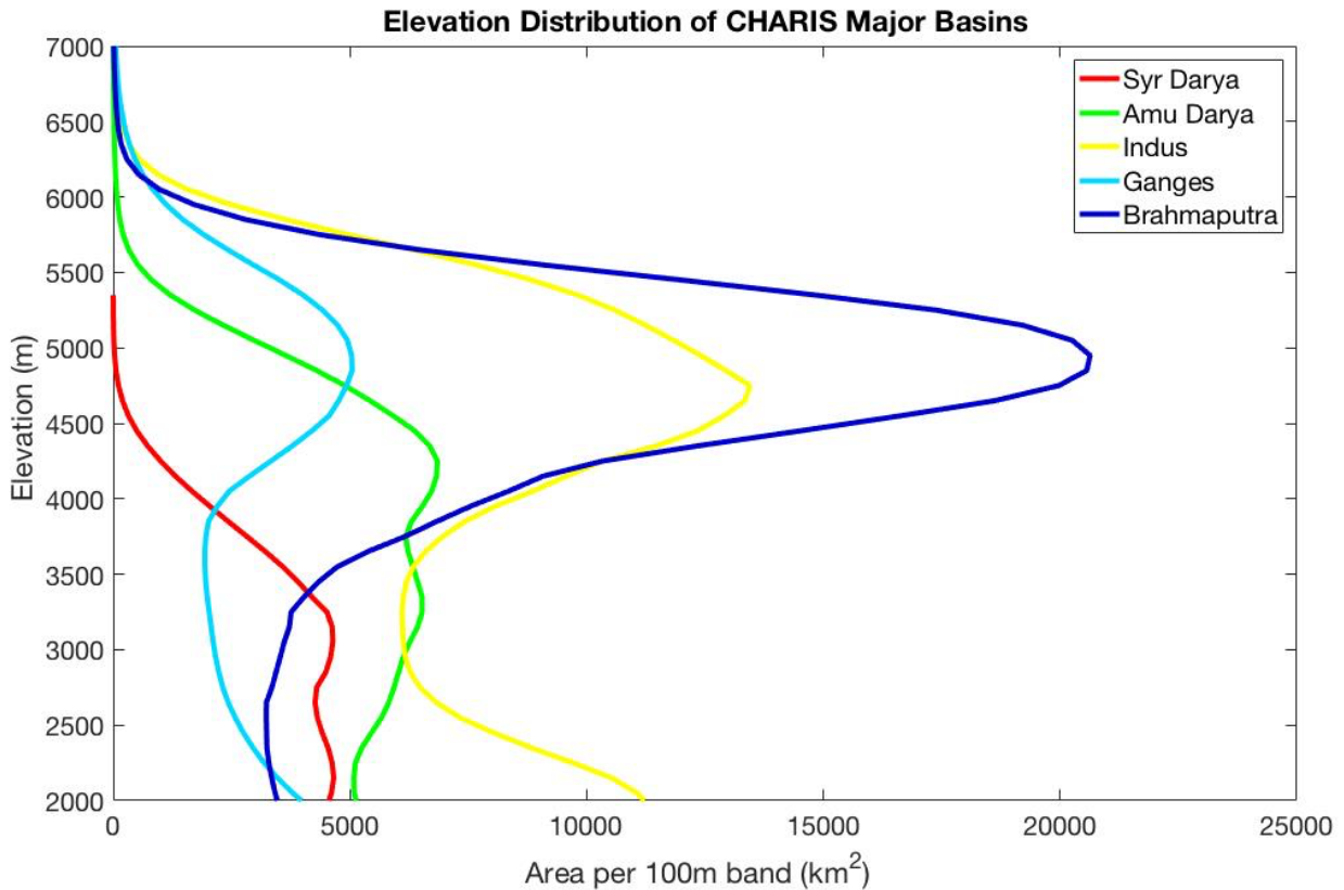
Fig. S1: Area-elevation distribution above 2000 m for the five major basins based on the Shuttle Radar Topography Mission (SRTM) digital elevation model (DEM) "SRTMGL3" (NASA JPL 2013).
