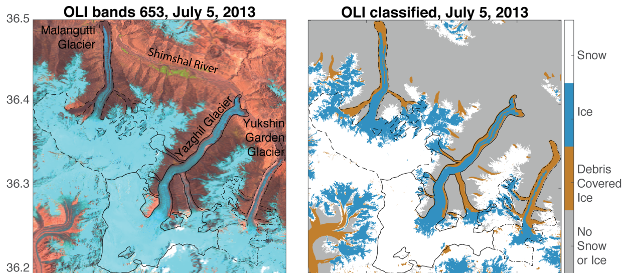
Fig. S4: Landsat 8 Operational Land Imager (OLI) false color composites (left) and classified maps (right) in the Hispar Muztagh region on July 05, 2013. Debris covered glaciers are identified using the Randolph Glacier Inventory (Arendt et al., 2013) for visual purposes only.
