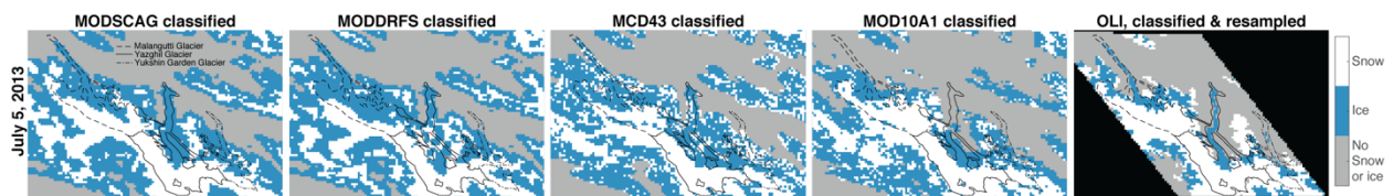
Fig. S5: Snow-Ice discrimination based on comparison with Landsat Operational Land Imager ( OLI ) for Moderate Resolution Imaging Spectroradiometer (MODIS) Snow Covered Area and Grain size (MODSCAG) (column 1), MODIS Dust Radiative Forcing in Snow (MODDRFS) (column 2), MCD43 (column 3), MOD10A1 (column 4), and coarsened Landsat (column 5) for July 5th, 2013
