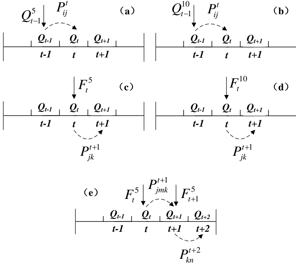
Fig. S1 Description of inflow processes in various models. (a) and (b) SDP- Q_{t-1} , (c) and (d) SDP- Q_t , (e) TS-BSDP.
