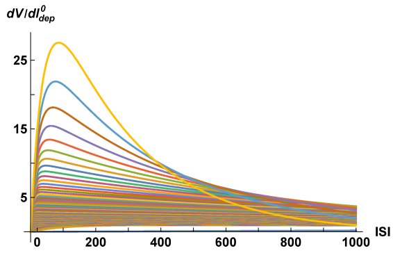
Suppl. Fig. 1 Plot of the derivative of V respect to I_{\text{dep}}^0 . Plot of the derivative (32) as function of t - t^0 obtained imposing the conditions (21) with a step of 0.01 for the parameter \delta .
