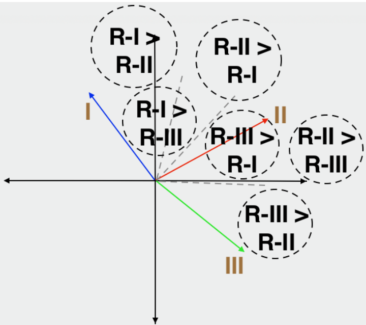
Supplementary Figure 4: Preferred decision subregions for > 2 classes. The class vectors are shown in red, blue and green and indicated in roman numerals, whereas the grey dotted lines are the respective bisectors of each pair of class vectors. The dotted circles label the preferred subregions.
