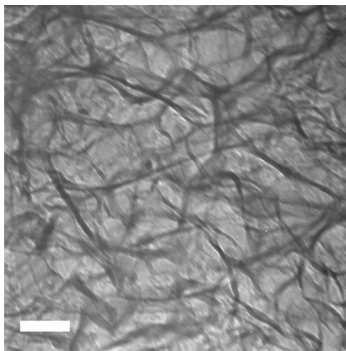
Figure S-2 Cryogenic Transmission Electron Microscopy (CTEM) image of 1.0 wt% K_{160}L_{40} gel (scale bar = 100 nm).
