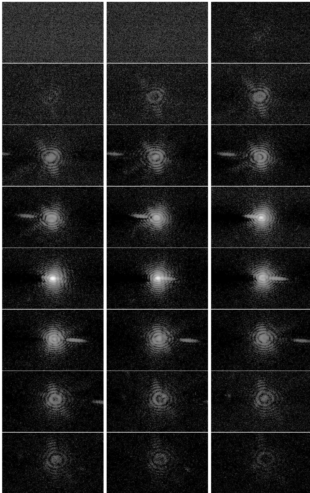
Figure S2: Raw coherent X-ray diffraction data measured for the Pb nanocrystal studied in this work. Every second frame of the rotation series of CCD images is shown. When stacked up, these constitute the 3D diffraction pattern of the sample.
