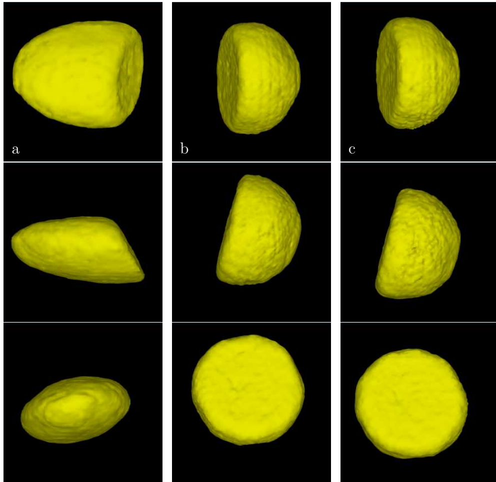
Figure S3: Isosurface views of the nanocrystal density, before (left column) and after (middle and right) performing the geometric correction. The middle and right columns were computed using different random starting phases. The top row is looking upstream towards the source, the middle row is a side view from below the crystal, and the bottom row is the view from the substrate.
