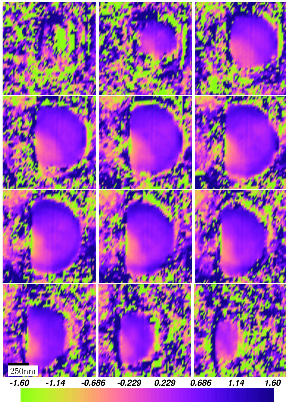
Figure S5: Sections of the real space phase map of the crystal. Phases corresponding to points with low density, i.e. outside the body of the crystal, have little meaning. The slices have a 69nm spacing.
