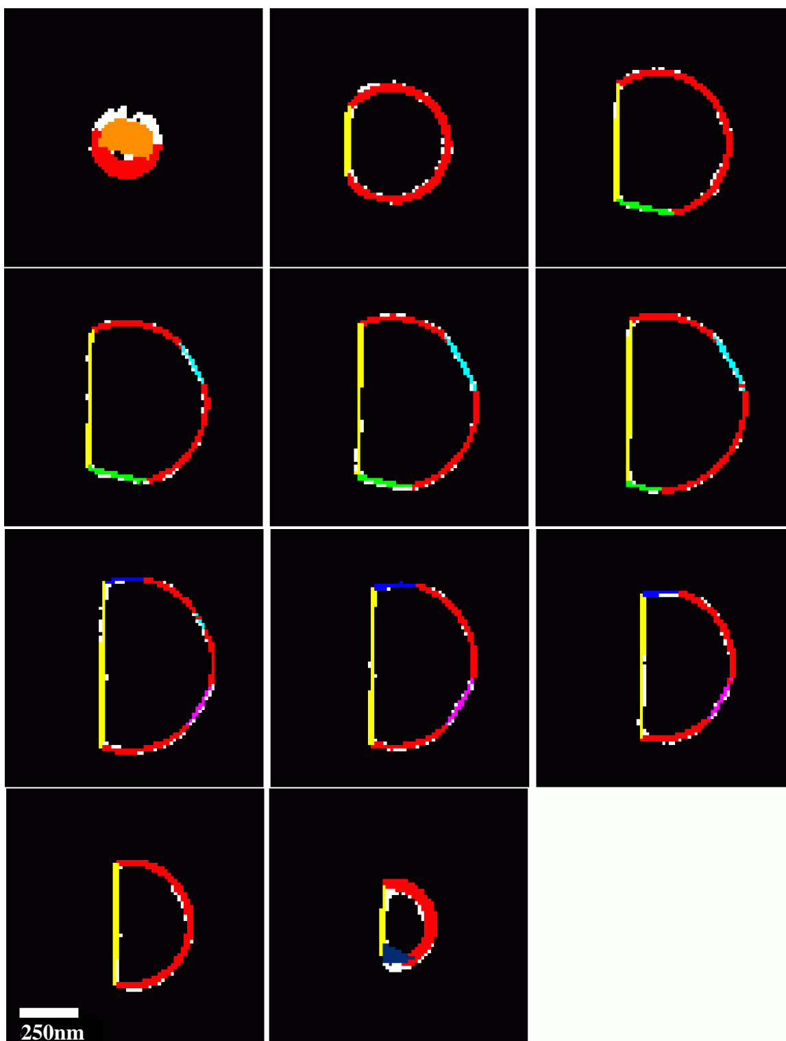
Figure S6: Least-square fits of the shape of the boundary of the real space density map of the crystal. The red curve is the best fitting sphere while the coloured straight lines represent the facets. Every fifth slice from the final 3D map is shown with 69nm spacing.
