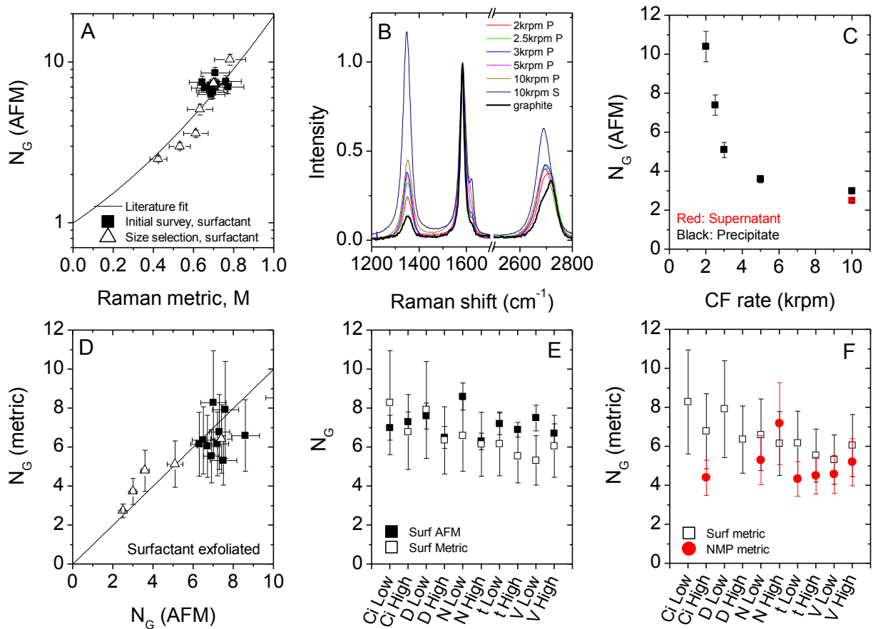
Figure S3.19: A) Mean number of monolayers per flake, N_G , measured by AFM for surfactant-exfoliated graphene plotted versus Raman thickness metric, M . The closed symbols represent the initial survey samples (e.g. figure S3.1), while the open symbols represent size-selected samples. The line is a plot of equation 3.5. B) Raman spectra for size-selected graphene. C) Flake thickness, N_G , measured by AFM plotted versus centrifugation speed used to select by size. D) Flake thickness, N_G , calculated using equation 3.5 plotted versus N_G as measured by AFM. E) Flake thickness, N_G , calculated using equation 3.5 plotted versus N_G as measured by AFM. F) Flake thickness, N_G , calculated using equation 3.5 plotted versus N_G as measured by AFM.
