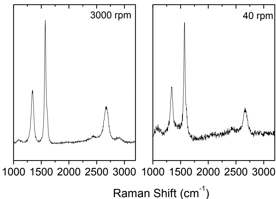
Figure S7.2: Raman spectra of material extracted from the Couette for two rotation speeds (after centrifugation). Left: After rotating at 3000 rpm for 60 minutes and Right: After rotating at 40 rpm for 60 minutes.
