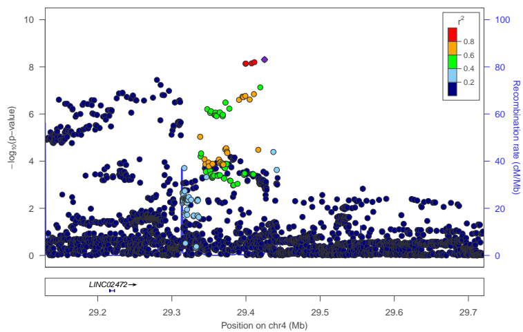
locus 144 rs2581458
