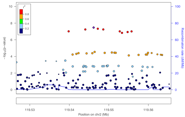
locus 69 rs773875123
