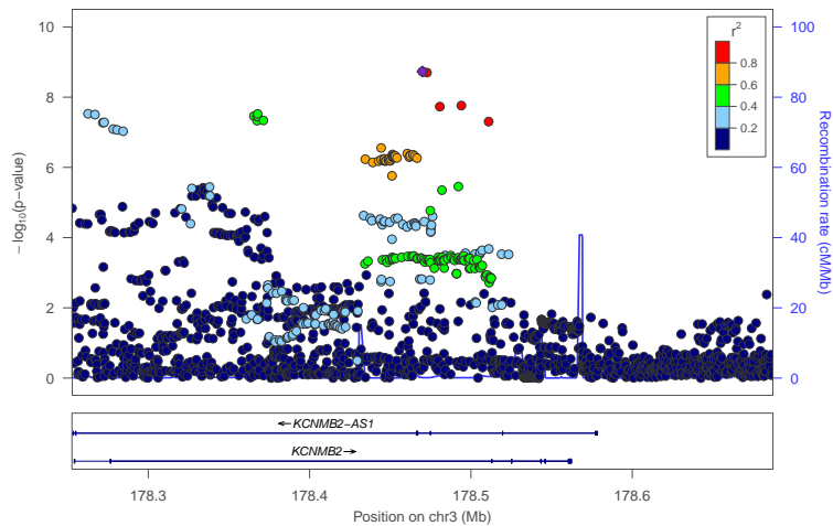
locus 134 rs6786798
