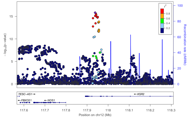
locus 408 rs585522
