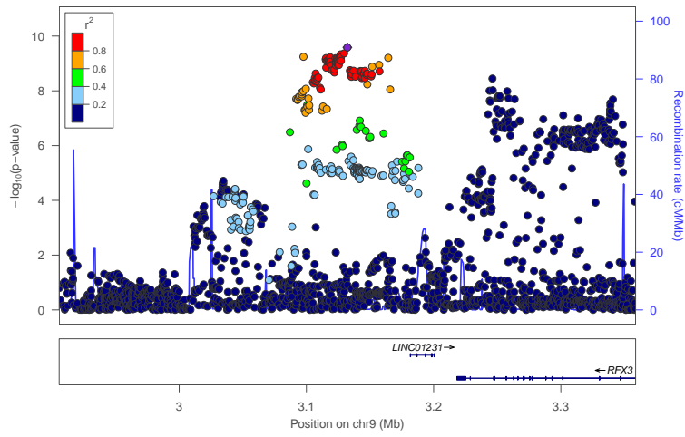
locus 305 rs7042696
