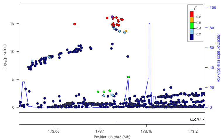
locus 132 rs4260410
