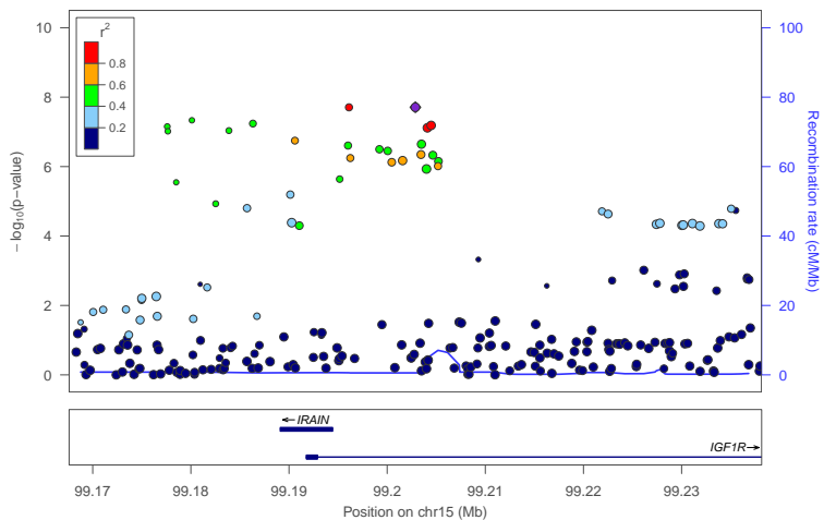
locus 470 rs11461440
