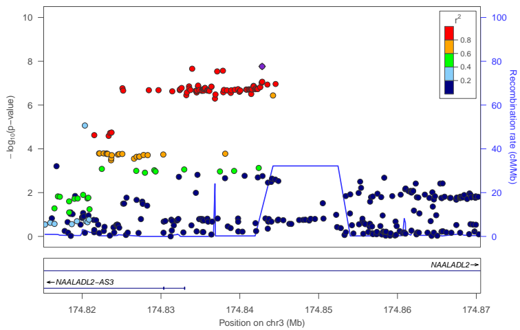
locus 133 rs2216427
