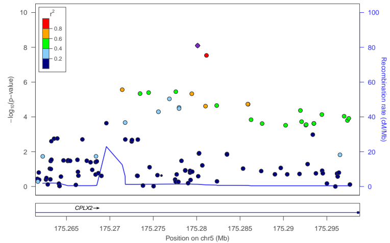
locus 201 rs4290977
