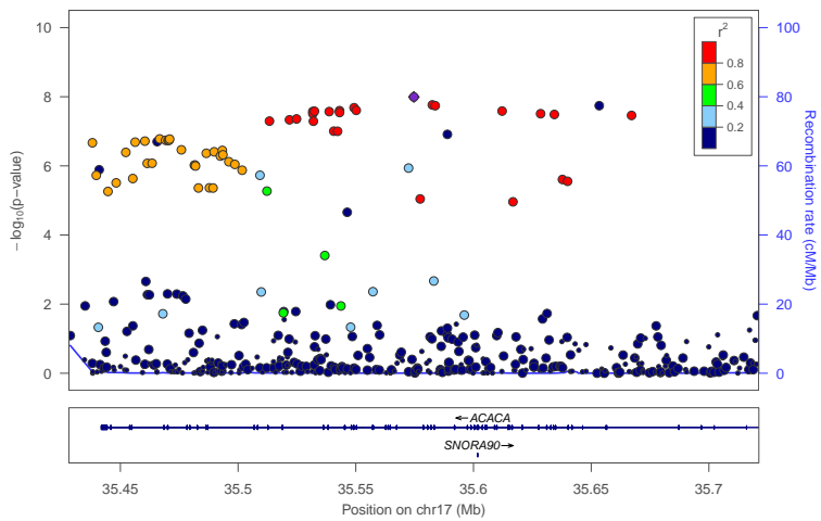
locus 502 rs4643373
