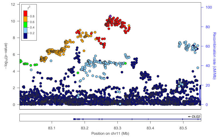
locus 376 rs1939252
