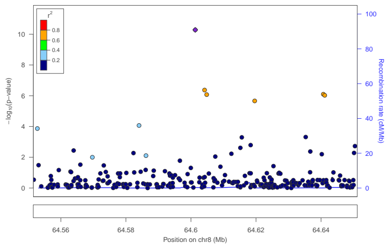
locus 287 rs10104523
