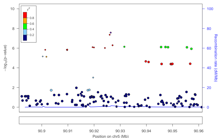
locus 176 rs4492142
