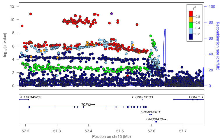
locus 457 rs2615252
