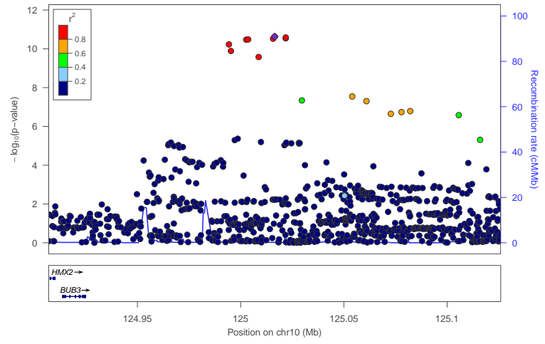
locus 358 rs9971199
