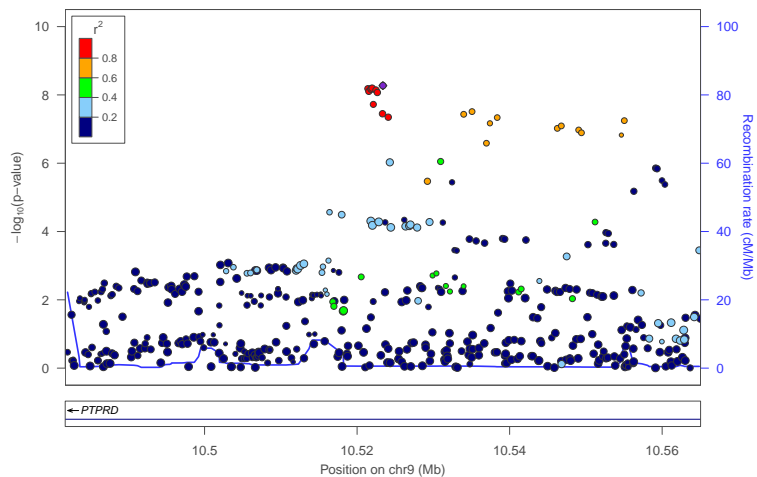
locus 309 rs10756553
