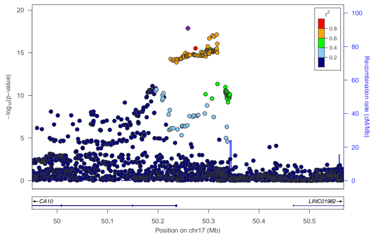
locus 505 rs6504568
