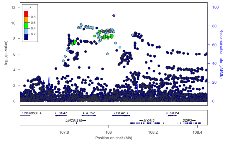
locus 119 rs9815484
