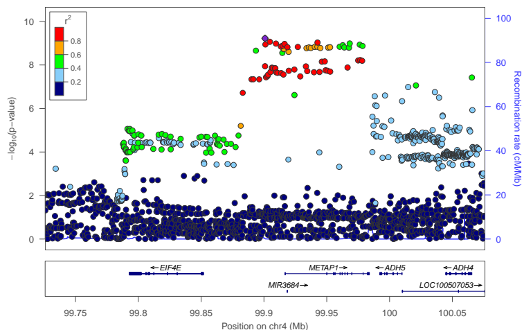
locus 152 rs11940529
