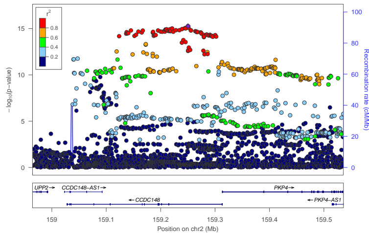
locus 79 rs1267070
