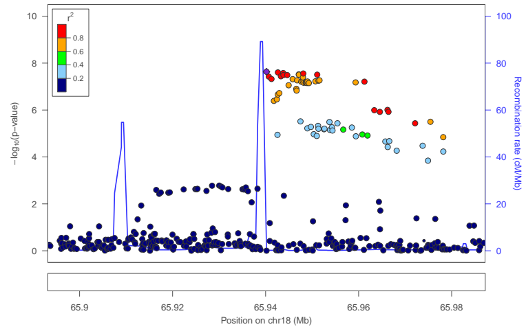
locus 520 rs12983032
