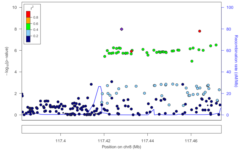
locus 302 rs2242090
