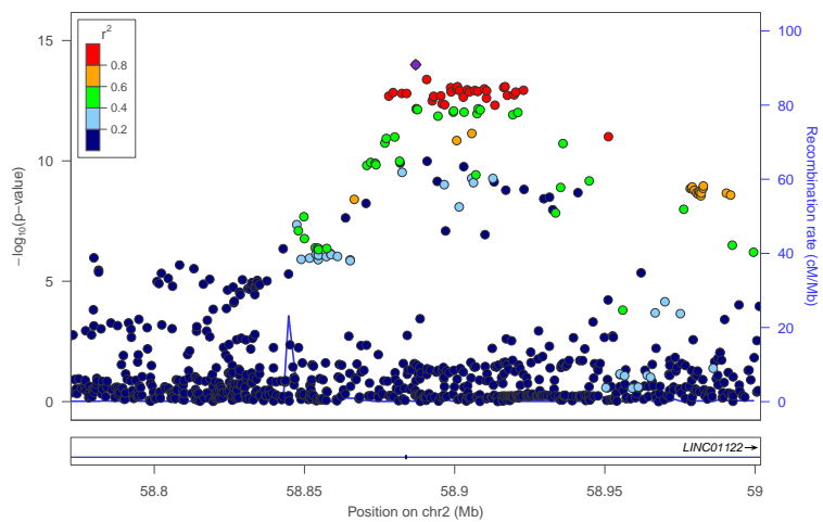
locus 56 rs13015703
