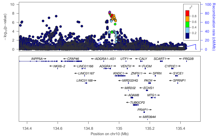
locus 361 rs7928823
