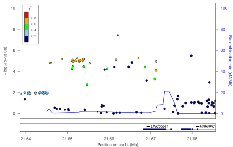
locus 434 rs10148610
