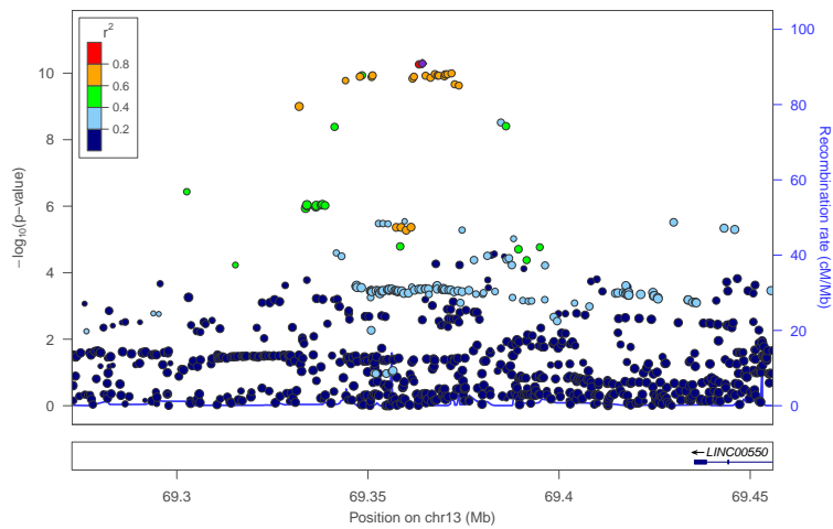
locus 421 rs7338765
