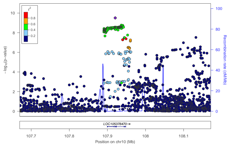
locus 354 rs72814942
