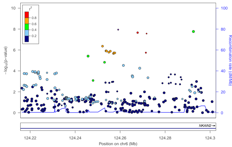
locus 230 rs1789695
