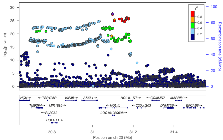
locus 536 rs6030790
