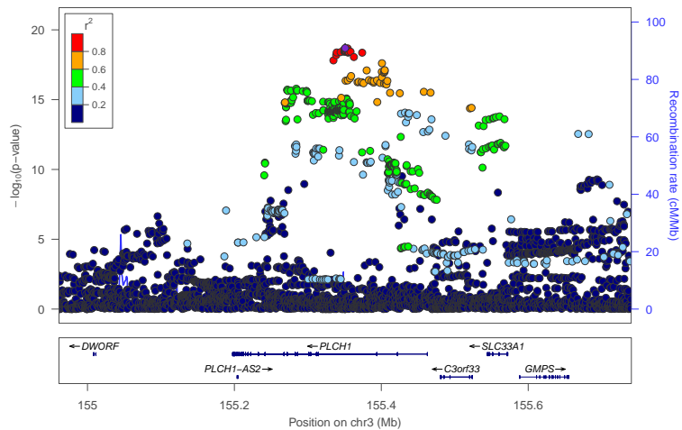
locus 127 rs34995891
