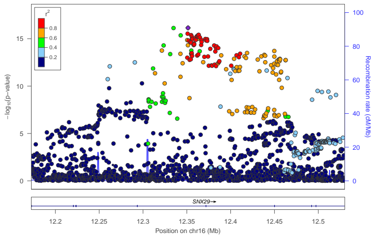
locus 474 rs111505982
