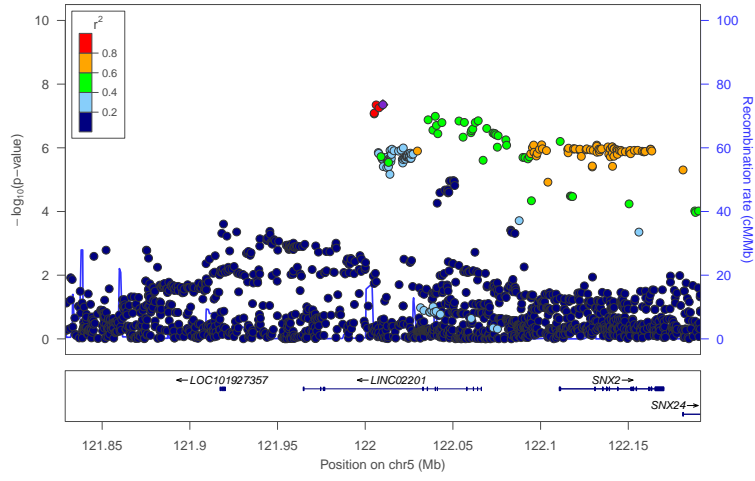
locus 188 rs10043722
