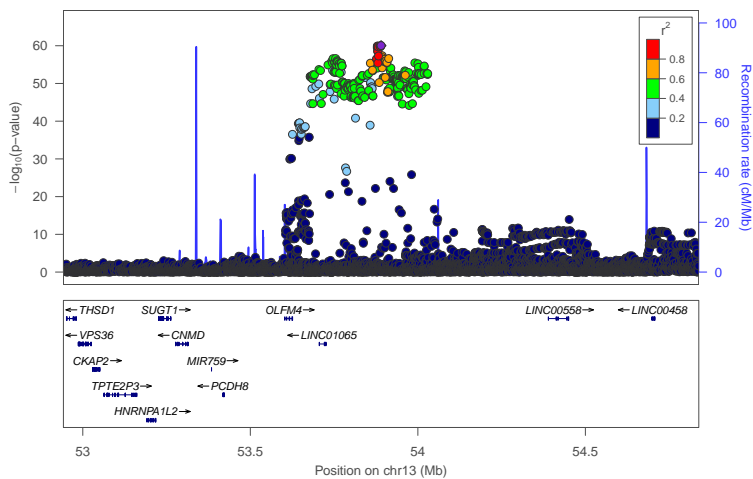
locus 416 rs9563886
