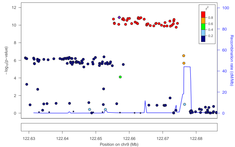
locus 322 rs10818399
