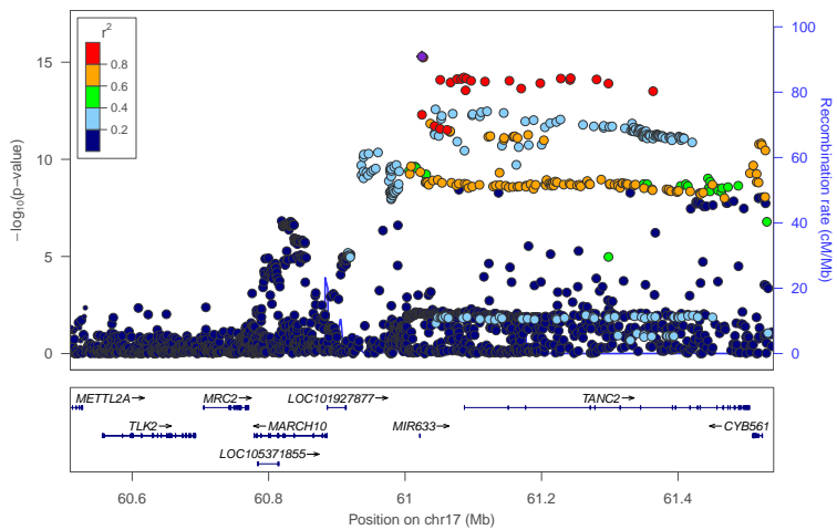
locus 506 rs323406
