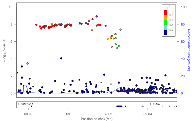
locus 110 rs115433278
