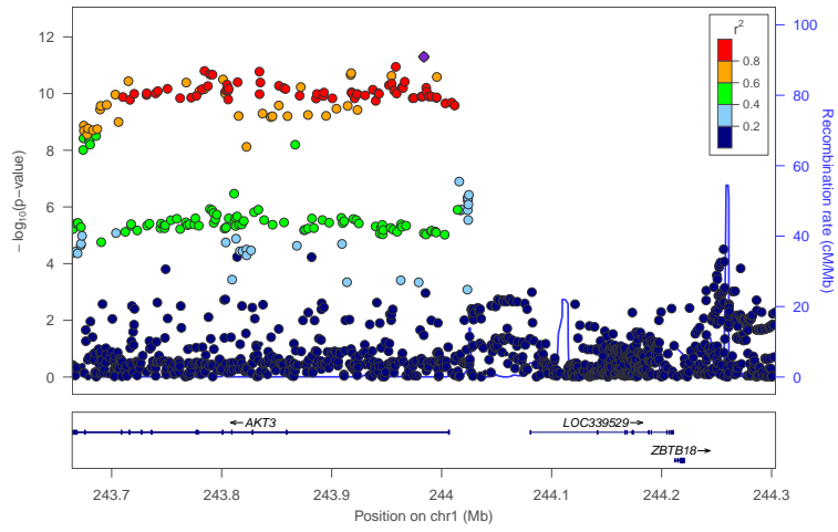
locus 44 rs10185535
