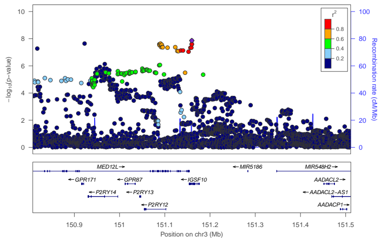
locus 125 rs13095140
