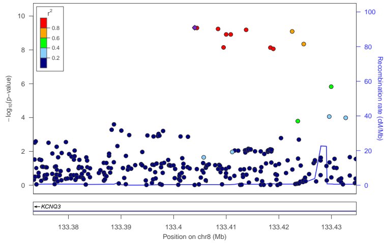
locus 303 rs17727688
