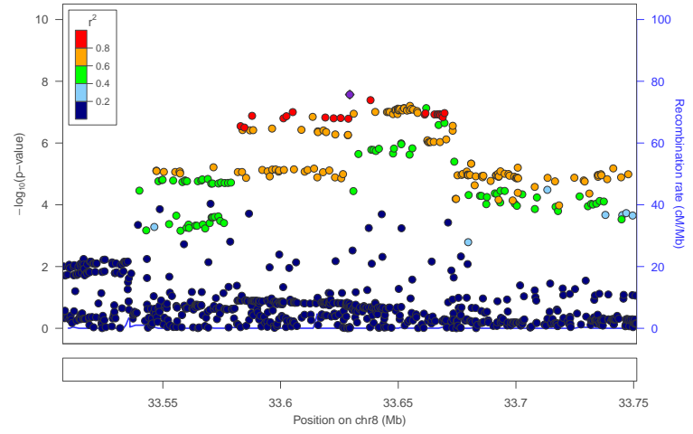
locus 280 rs5891160
