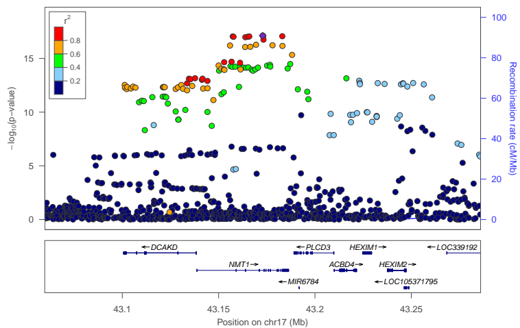
locus 503 rs9889282
