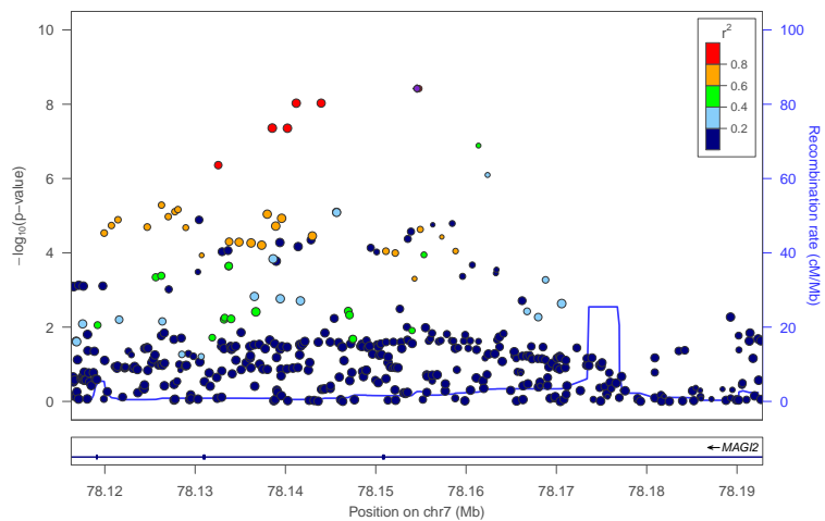
locus 250 rs1468774
