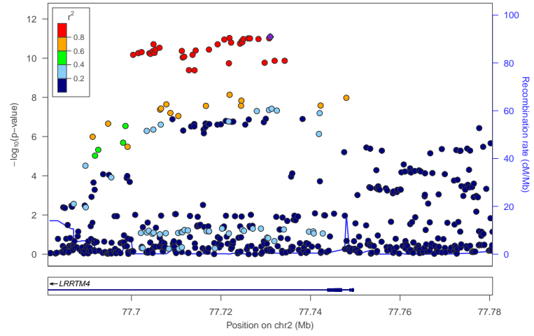
locus 63 rs6735012
