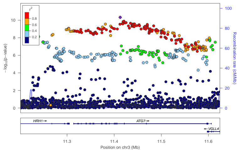
locus 102 rs4858241
