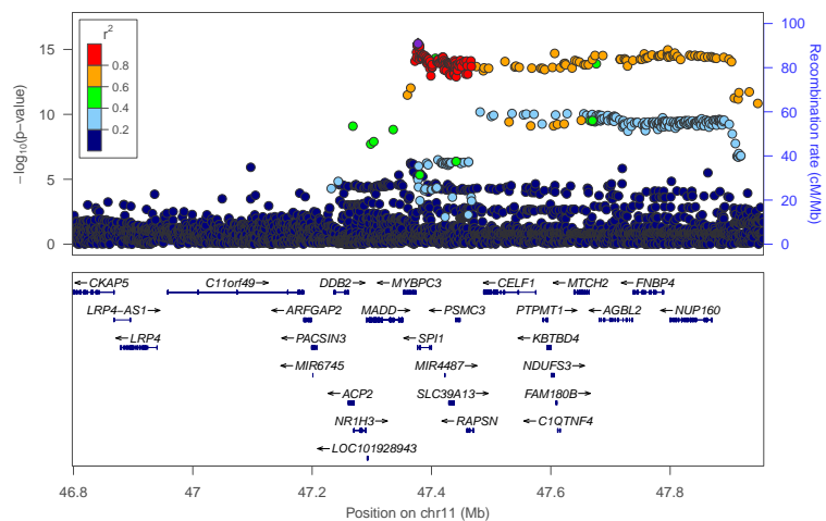
locus 370 rs12790660
