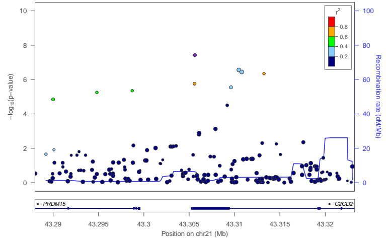
locus 547 rs147970828
