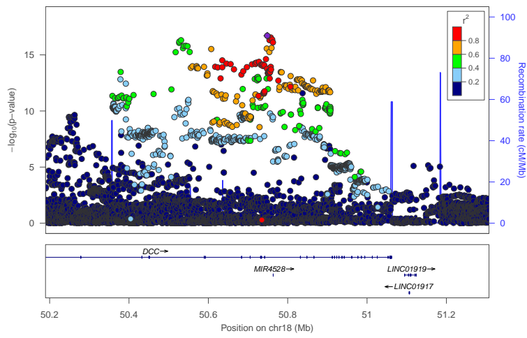
locus 517 rs2271731
