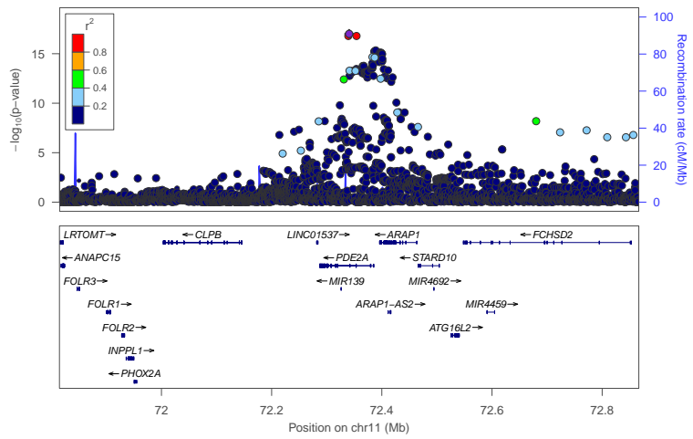
locus 375 rs519778
