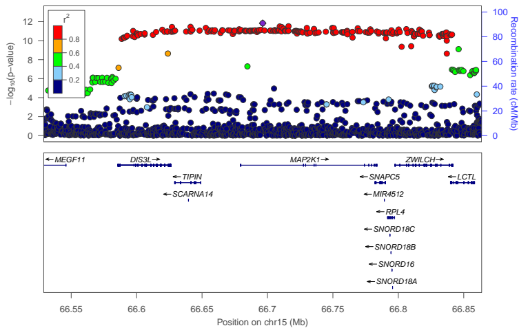
locus 458 rs11856510
