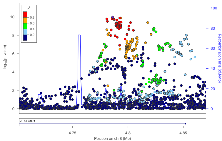
locus 271 rs4831647
