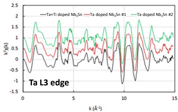
Figure S1. k^2 weighted \chi(k) data for the Ta L3 edge.
