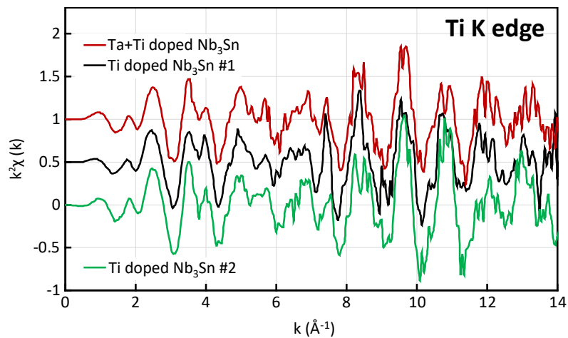
Figure S2. k^2 weighted \chi(k) data for the Ti K edge.
