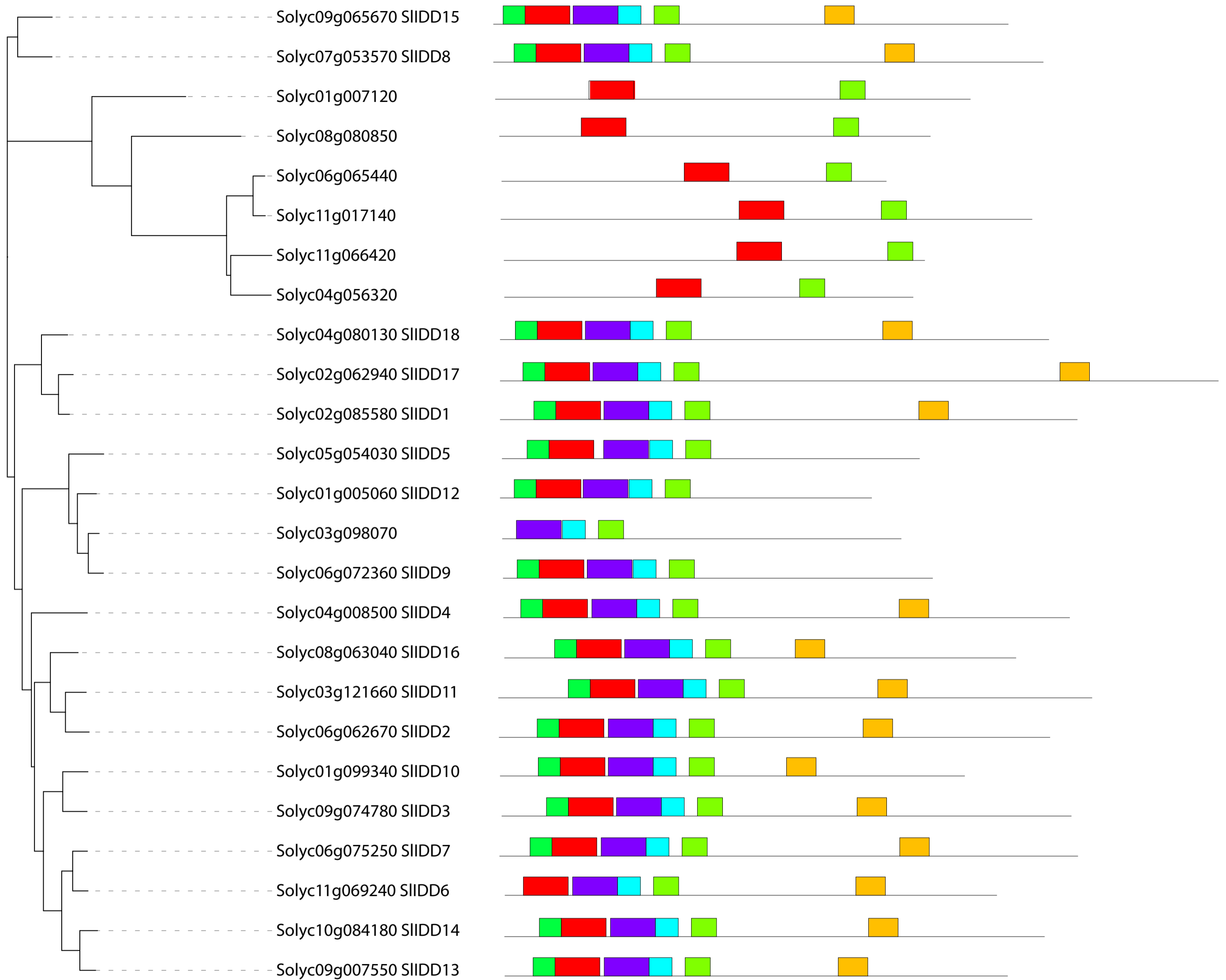
Figure S3. Motif analysis of Tomato IDD-like transcription factors. Sequences with 4 conserved C-terminus motifs were named as IDDs .
