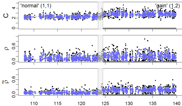
(a) N/G: normal (1,1) / gain (1,2)
