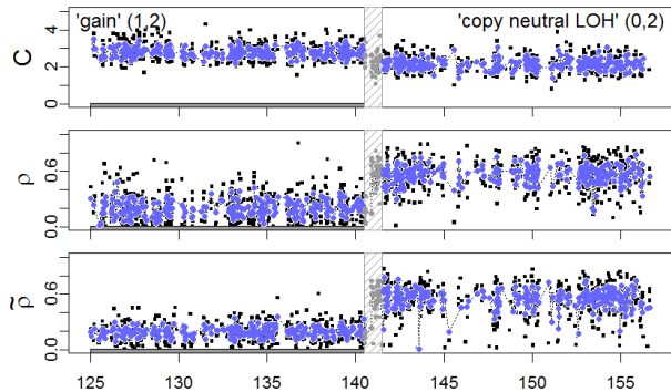
(b) G/L: gain (1,2) / copy-neutral LOH (0,2)
